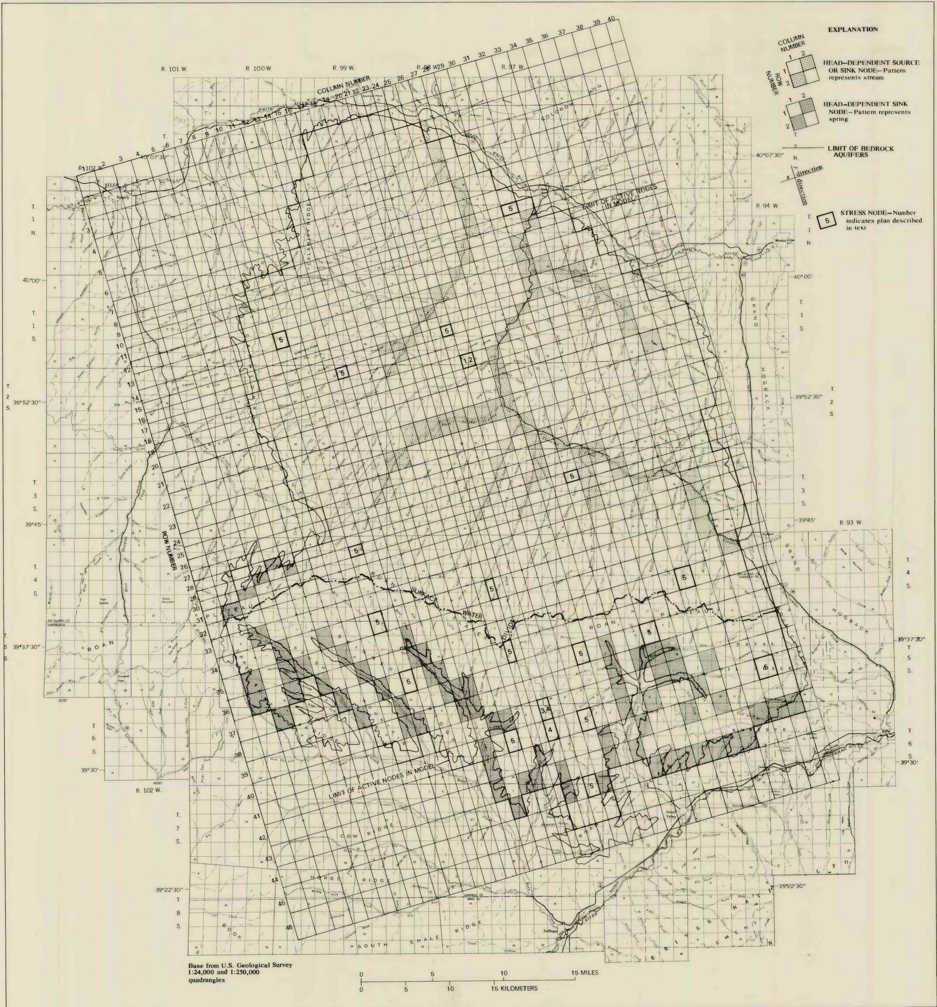
MAP SHOWING GRID FOR MATHEMATICAL MODEL OF THE HYDROLOGIC SYSTEM
