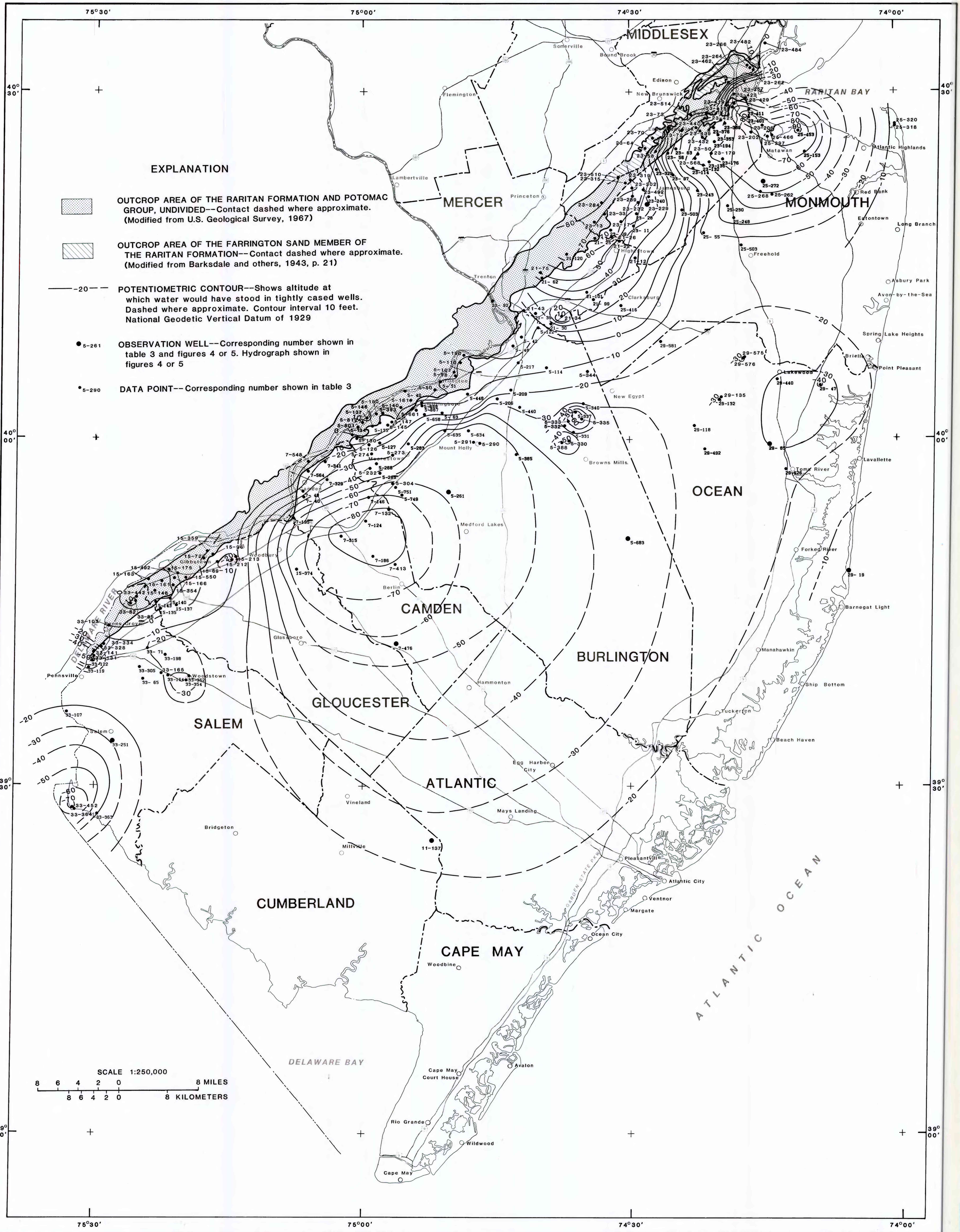
POTENTIOMETRIC SURFACE OF THE MIDDLE AQUIFER AND UNDIFFERENTIATED PART OF THE POTOMAC-RARITAN-MAGOTHY AQUIFER SYSTEM, 1983
