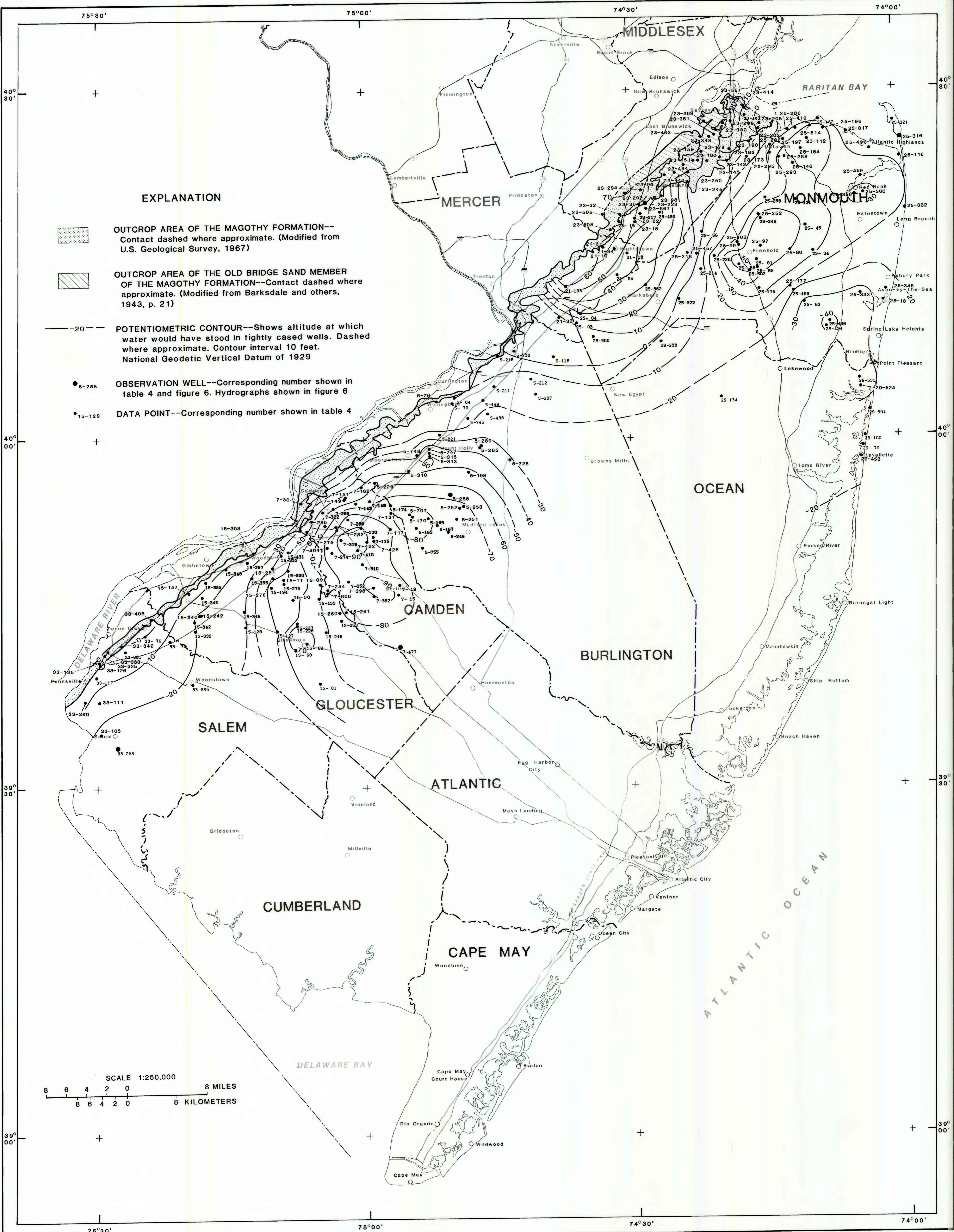
POTENTIOMETRIC SURFACE OF THE UPPER AQUIFER OF THE POTOMAC-RARITAN-MAGOTHY AQUIFER SYSTEM, 1983
