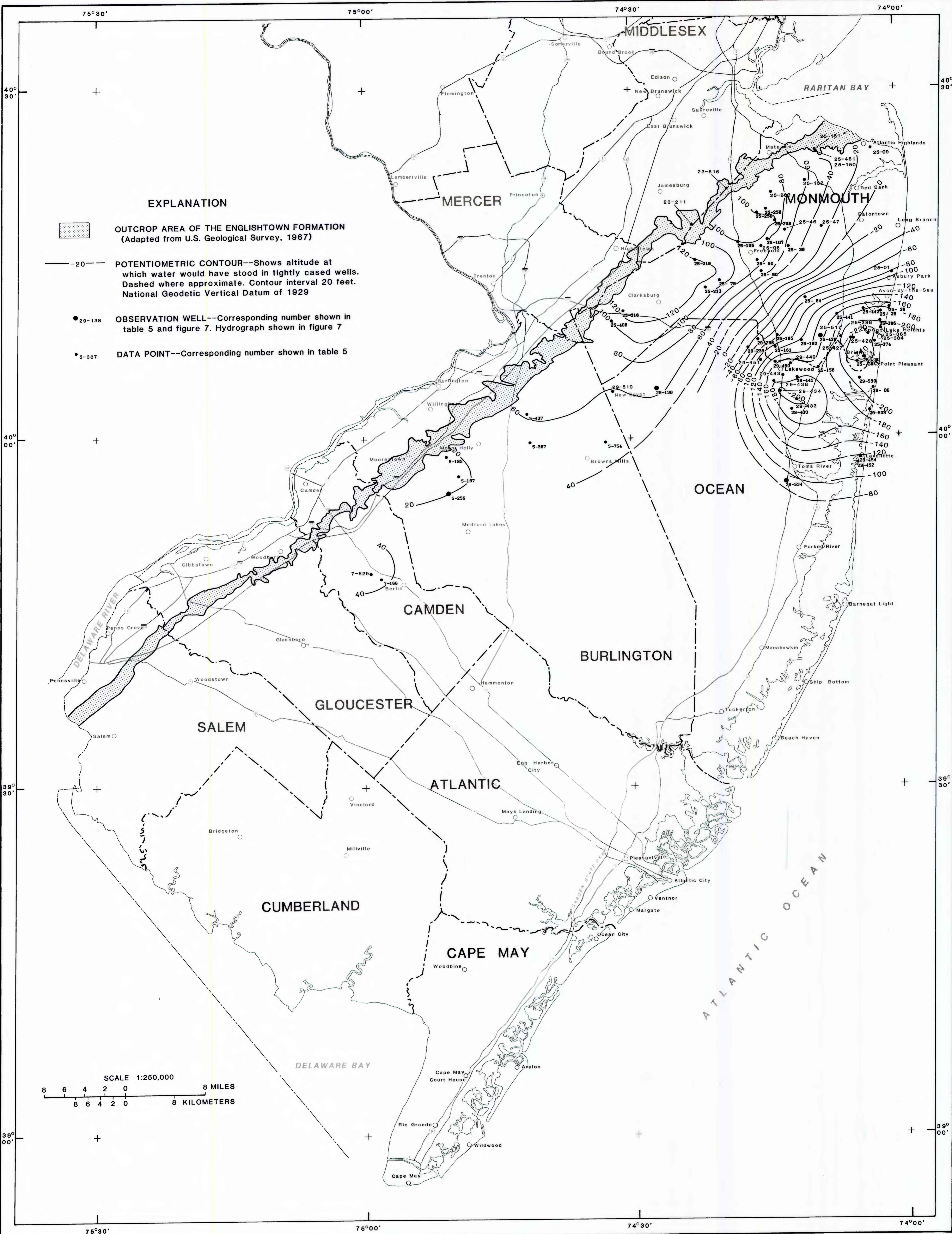
POTENTIOMETRIC SURFACE OF THE ENGLISHTOWN AQUIFER SYSTEM, 1983
