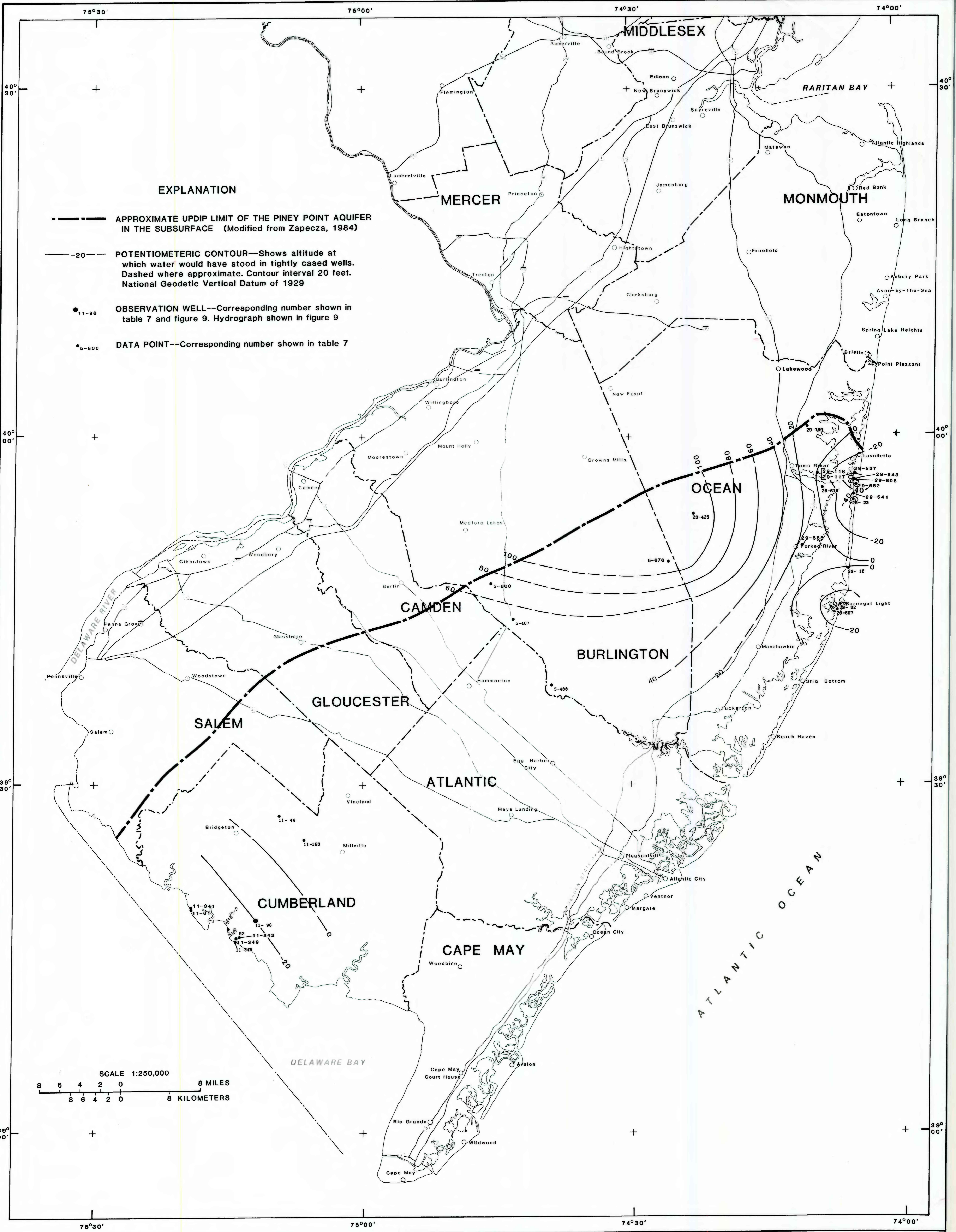
POTENTIOMETRIC SURFACE OF THE PINEY POINT AQUIFER, 1983
