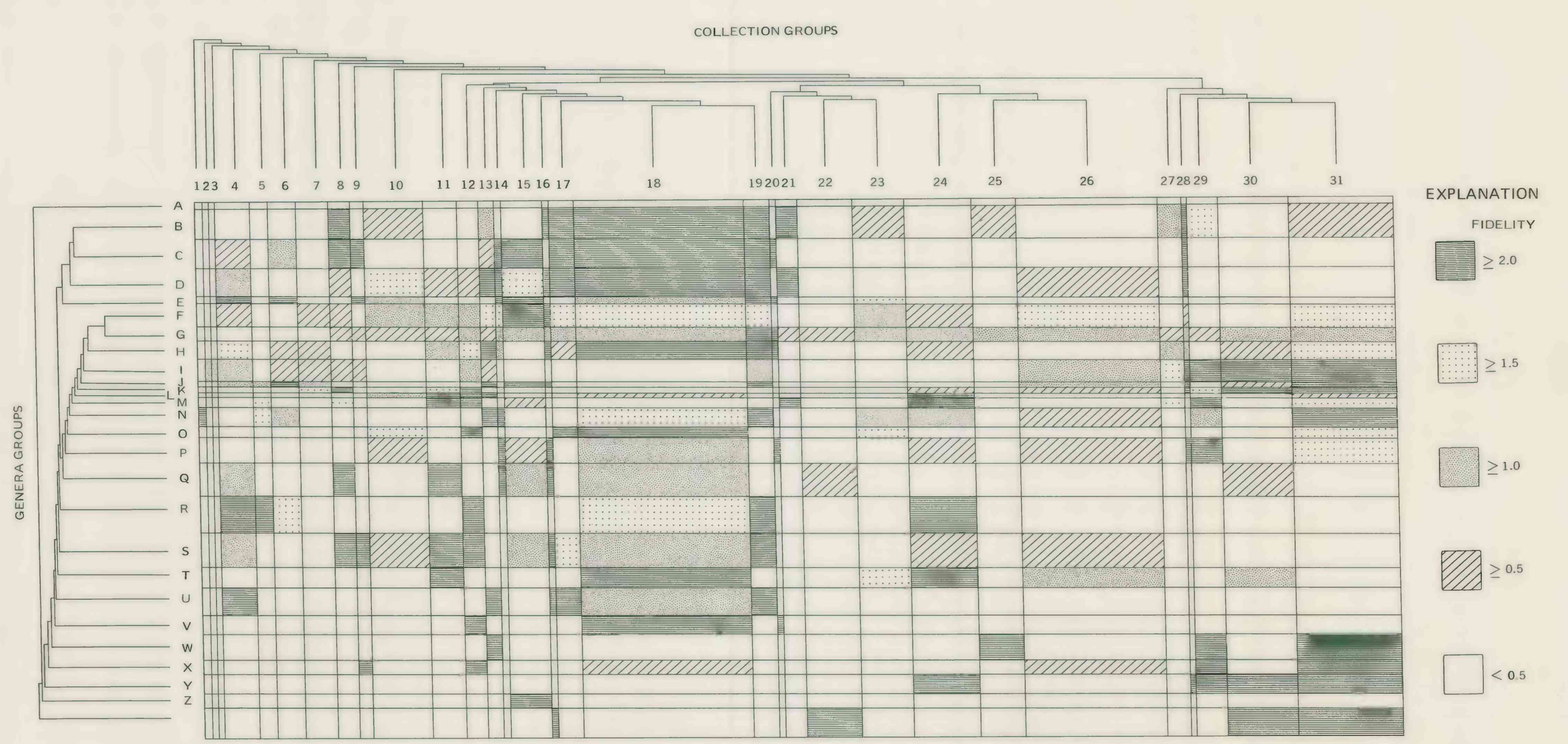
F—Diagram of nodal fidelity for data from the Tennessee River basin (based on the analysis of phytoplankton data at four stations for the period 1974-81).
