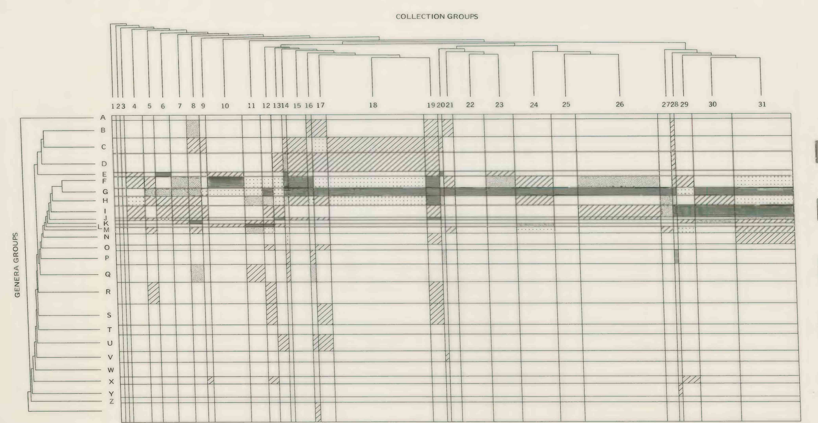
E—Diagram of nodal constancy for data from the Tennessee River basin (based on the analysis of phytoplankton data at four stations for the period 1974-81).
