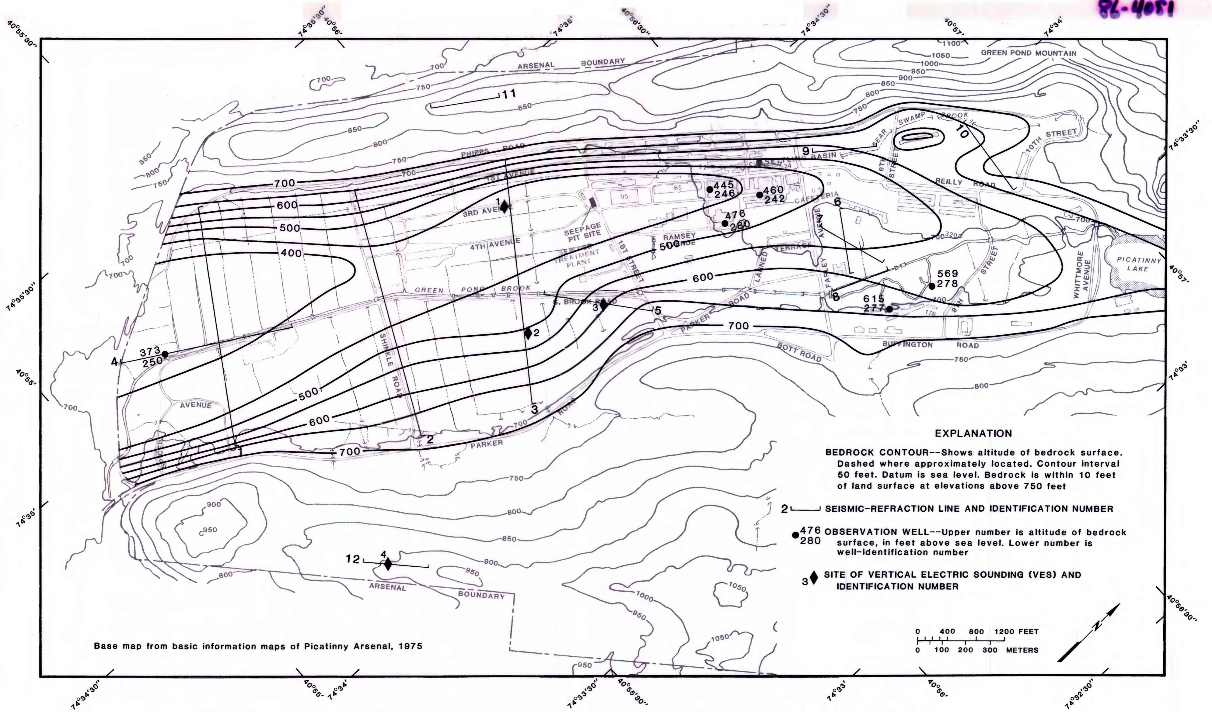
Figure 4.--Configuration of the bedrock surface and the location of seismic-refraction and electric-resistivity measurements.
