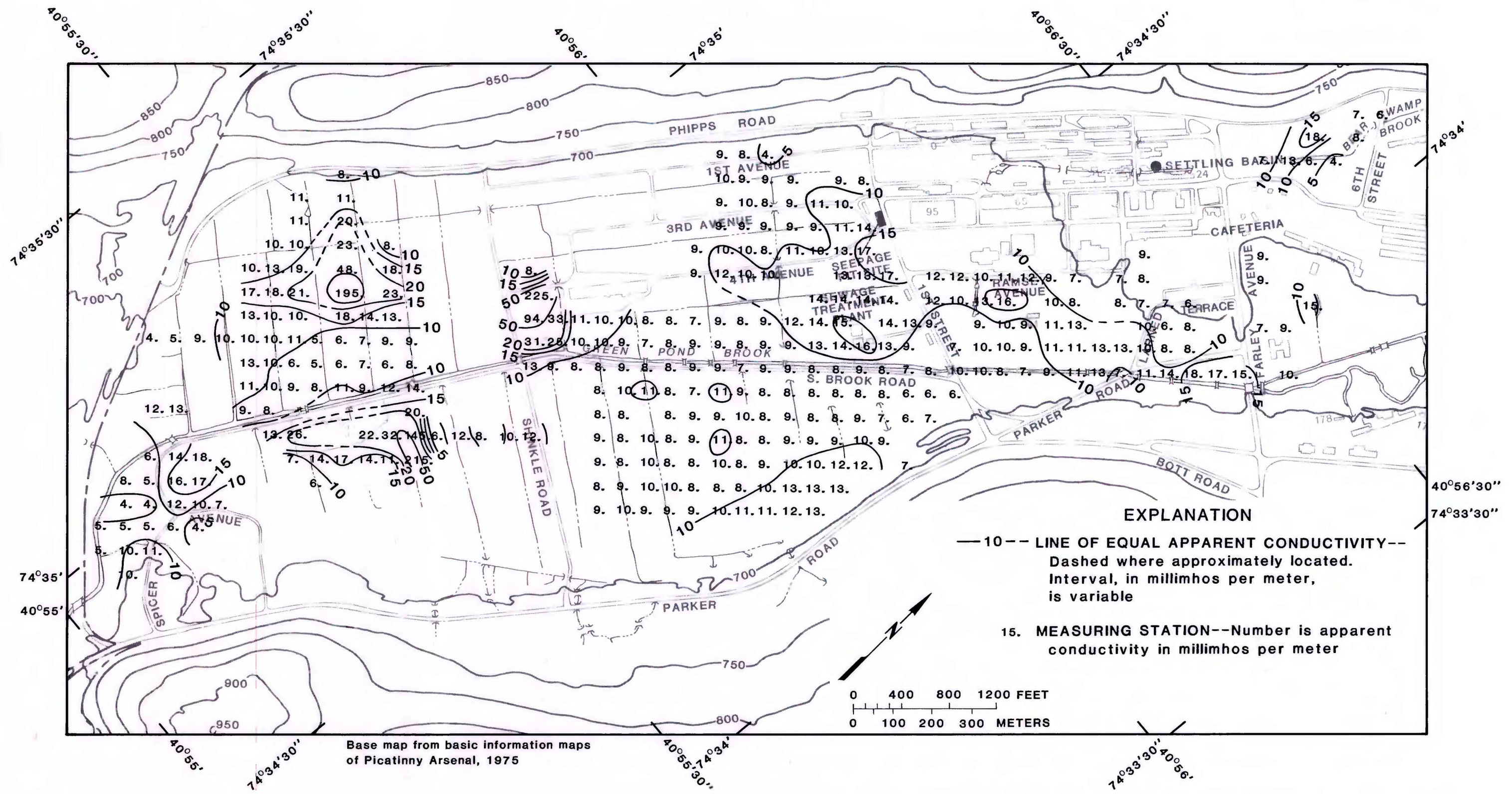
Figure 8.--Distribution of apparent conductivity values collected in the horizontal-dipole configuration with 32.8 feet between coils, June 1983.
