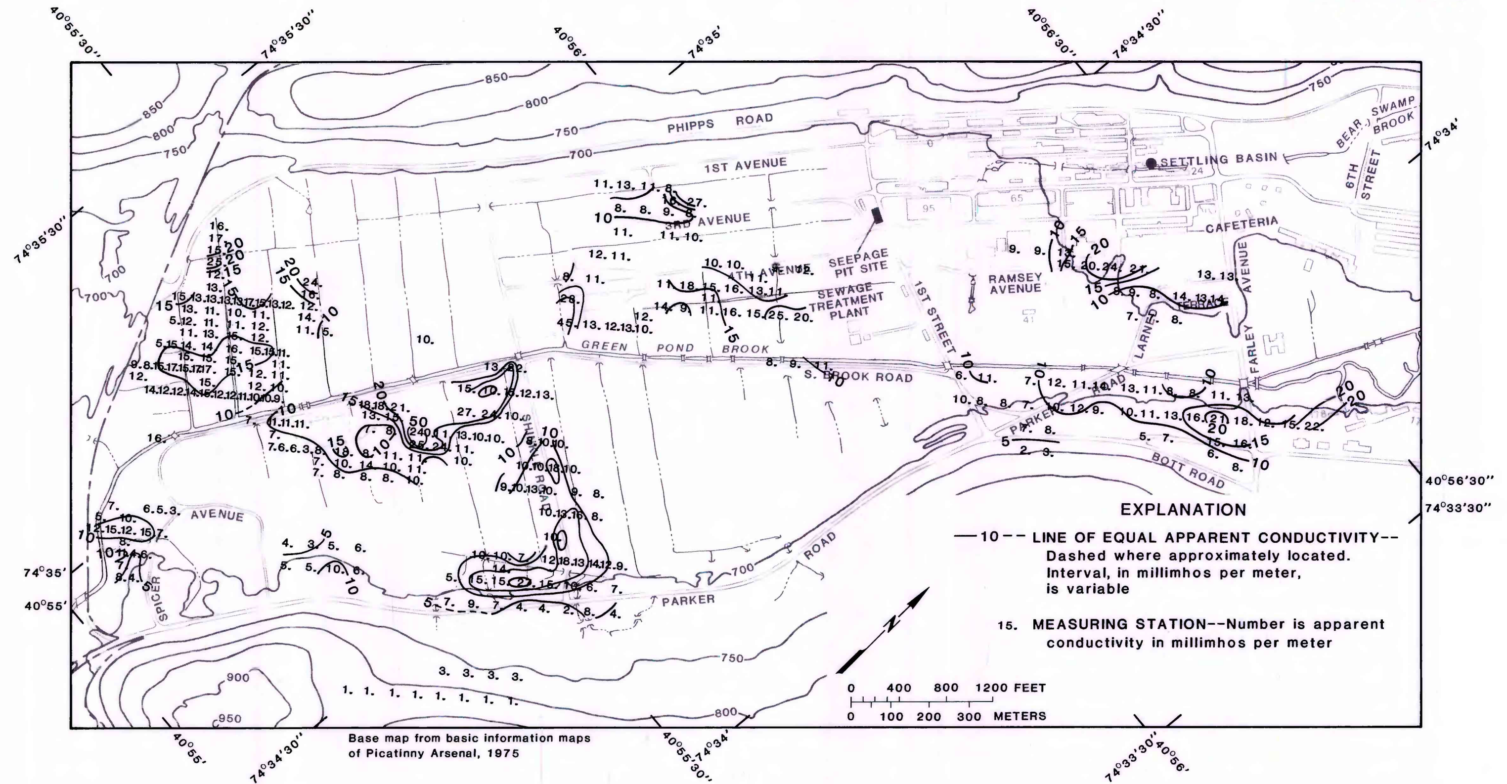
Figure 10.--Distribution of apparent conductivity values collected in the horizontal-dipole configuration with 12 feet between coils, June 1983.
