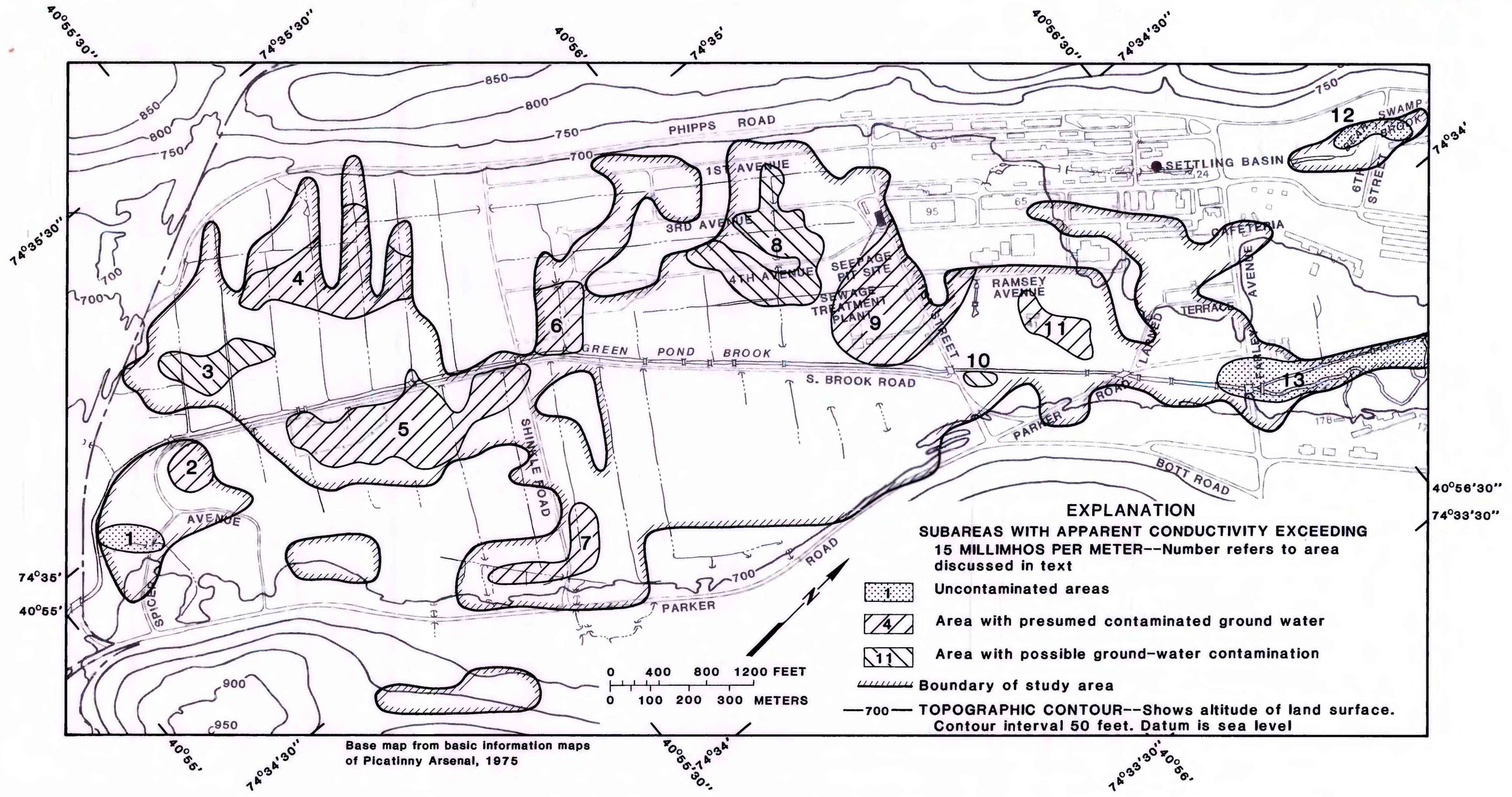
Figure 11.--Map showing boundary of apparent-conductivity surveys and subareas with high apparent conductivity.
