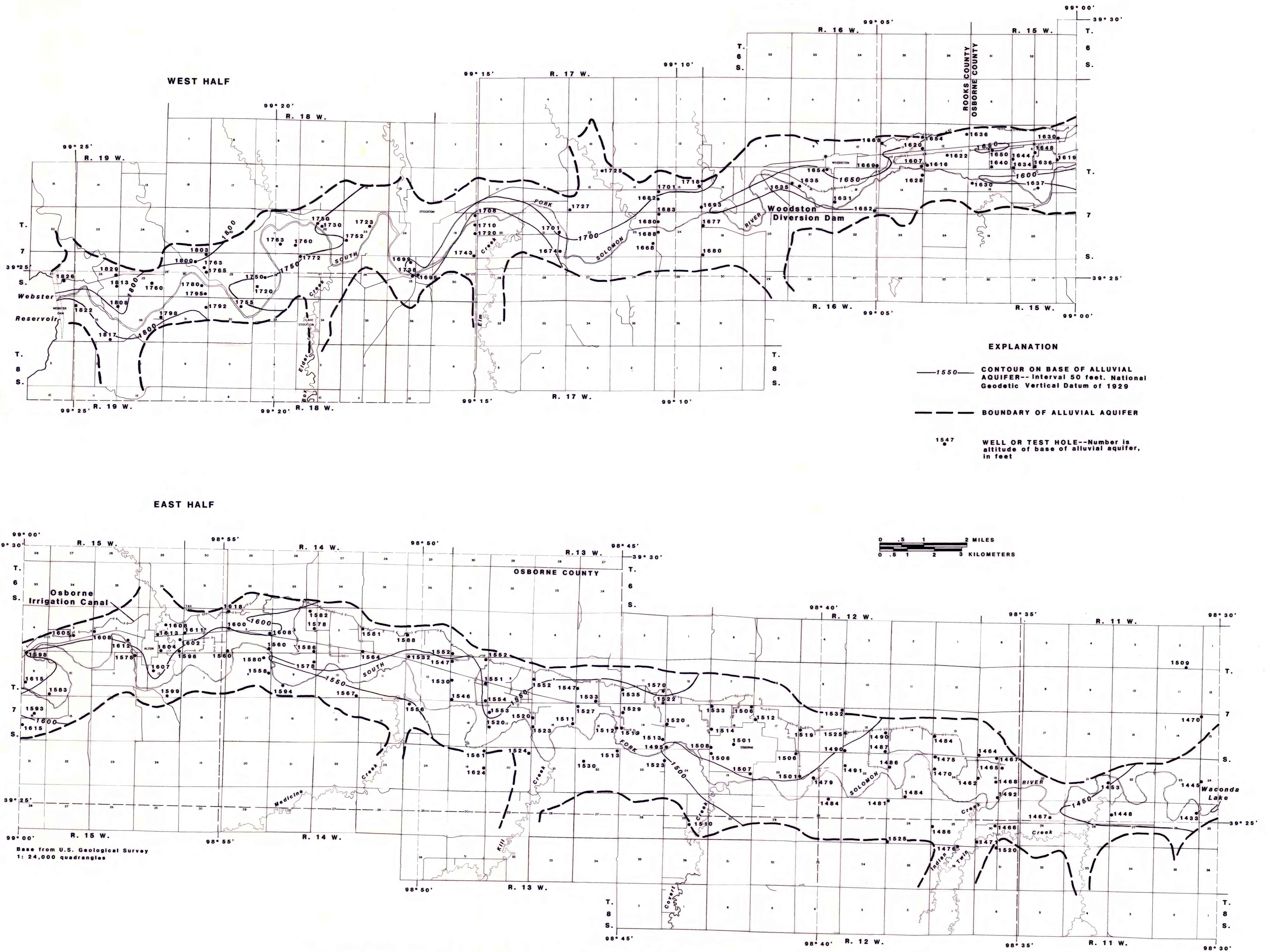
MAP SHOWING AREAL EXTENT AND CONFIGURATION OF BASE OF ALLUVIAL AQUIFER, SOUTH FORK SOLOMON RIVER VALLEY, WEBSTER RESERVOIR TO WACONDA LAKE, NORTH-CENTRAL KANSAS
