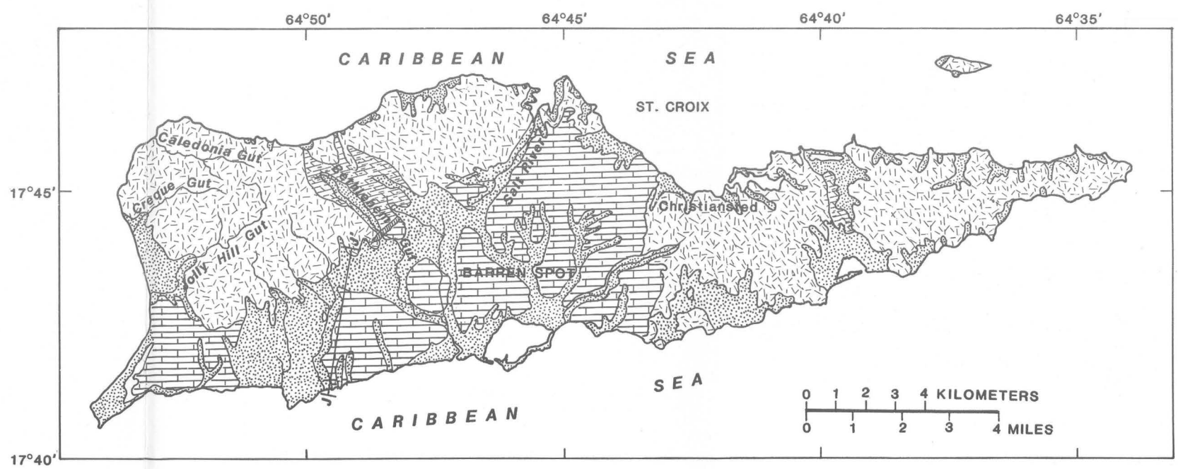
Plate 2.--Generalized surficial geology of the U.S. Virgin Islands.
