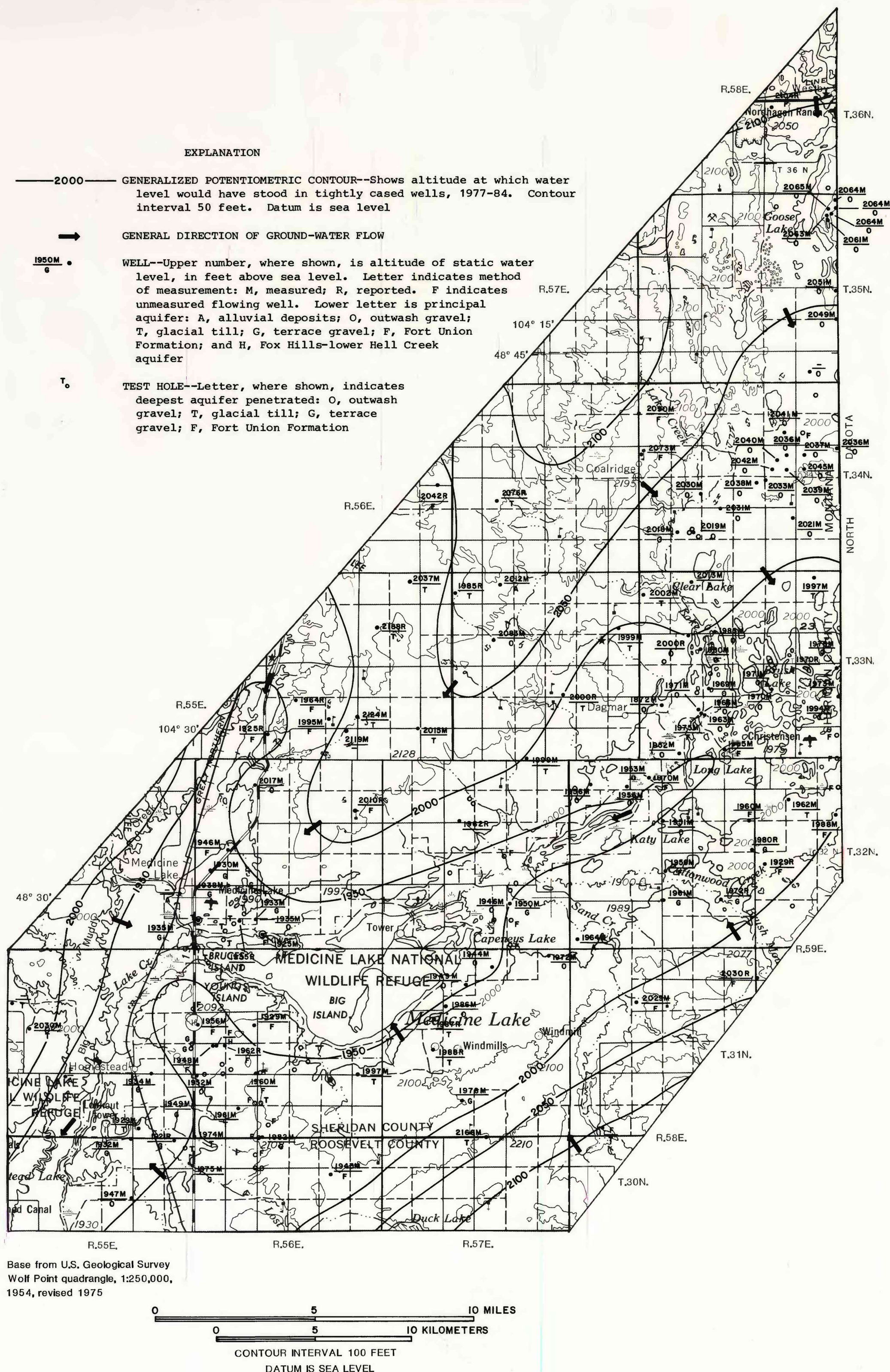
MAP SHOWING GENERALIZED POTENTIOMETRIC SURFACE, DIRECTION OF GROUND-WATER FLOW, AQUIFERS, AND LOCATION OF WELLS AND TEST HOLES IN AND NEAR THE ANCESTRAL MISSOURI RIVER VALLEY, NORTHEASTERN MONTANA
