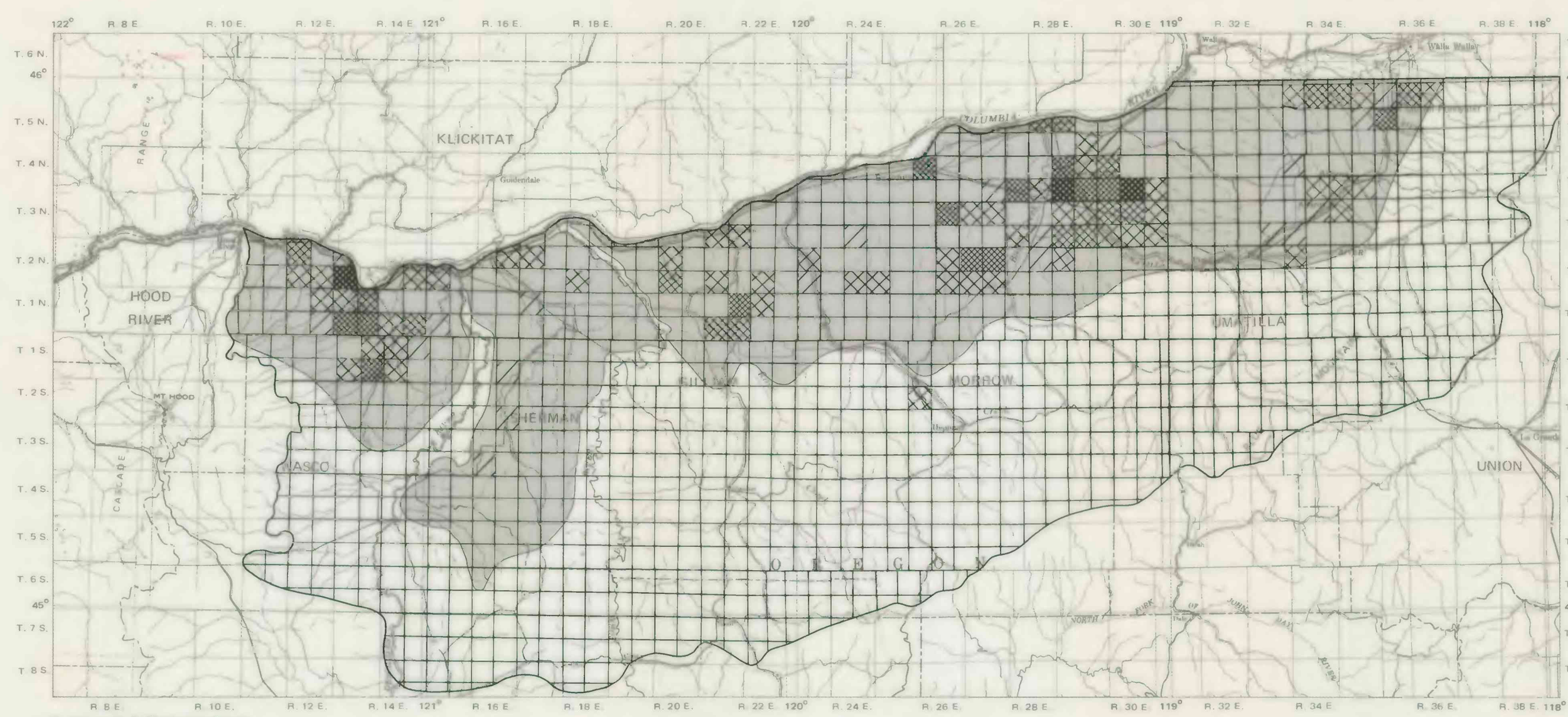
WANAPUM UNIT
