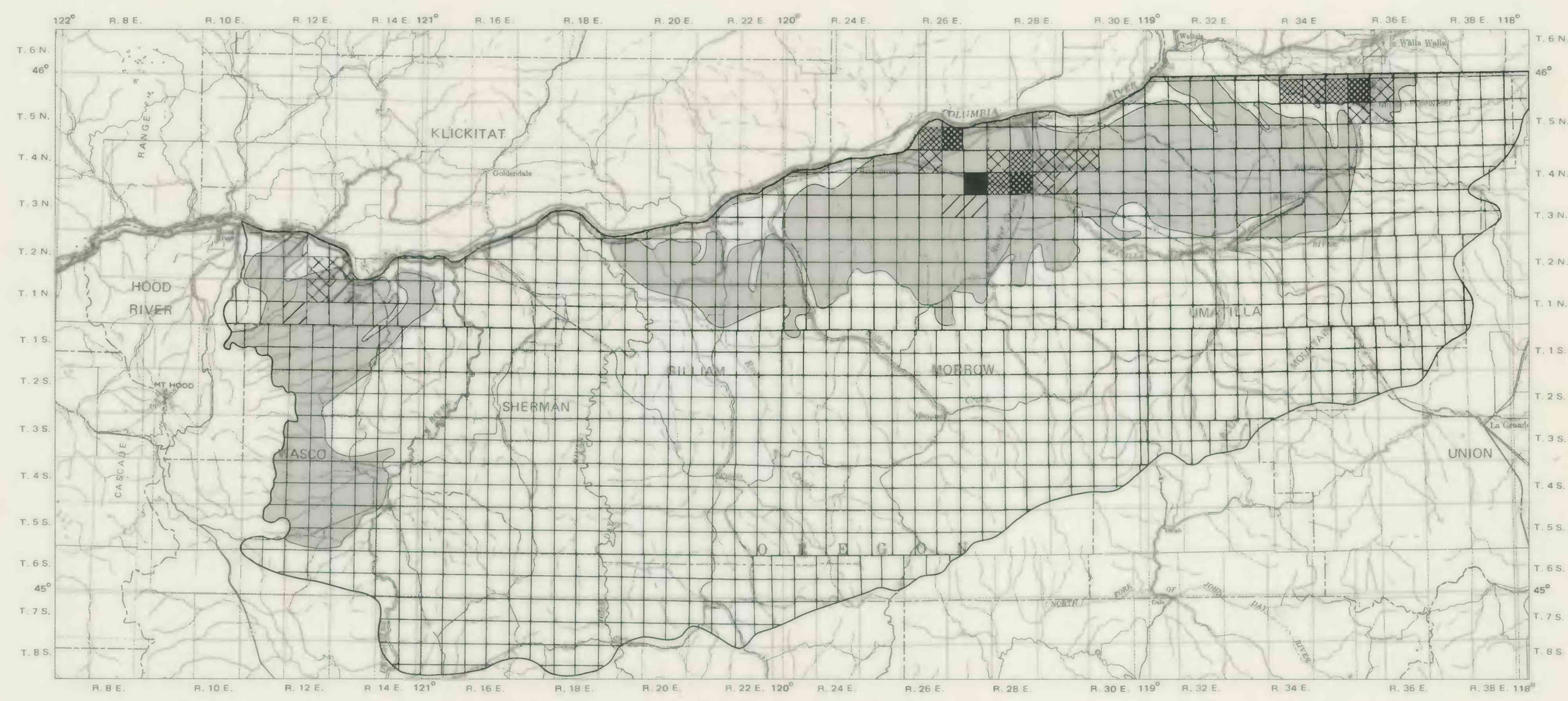
OVERBURDEN UNIT
