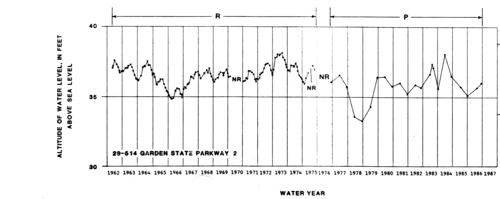
HYDROGRAPHS OF GROUND-WATER LEVELS IN THE KIRKWOOD-COHANSEY AQUIFER SYSTEM
