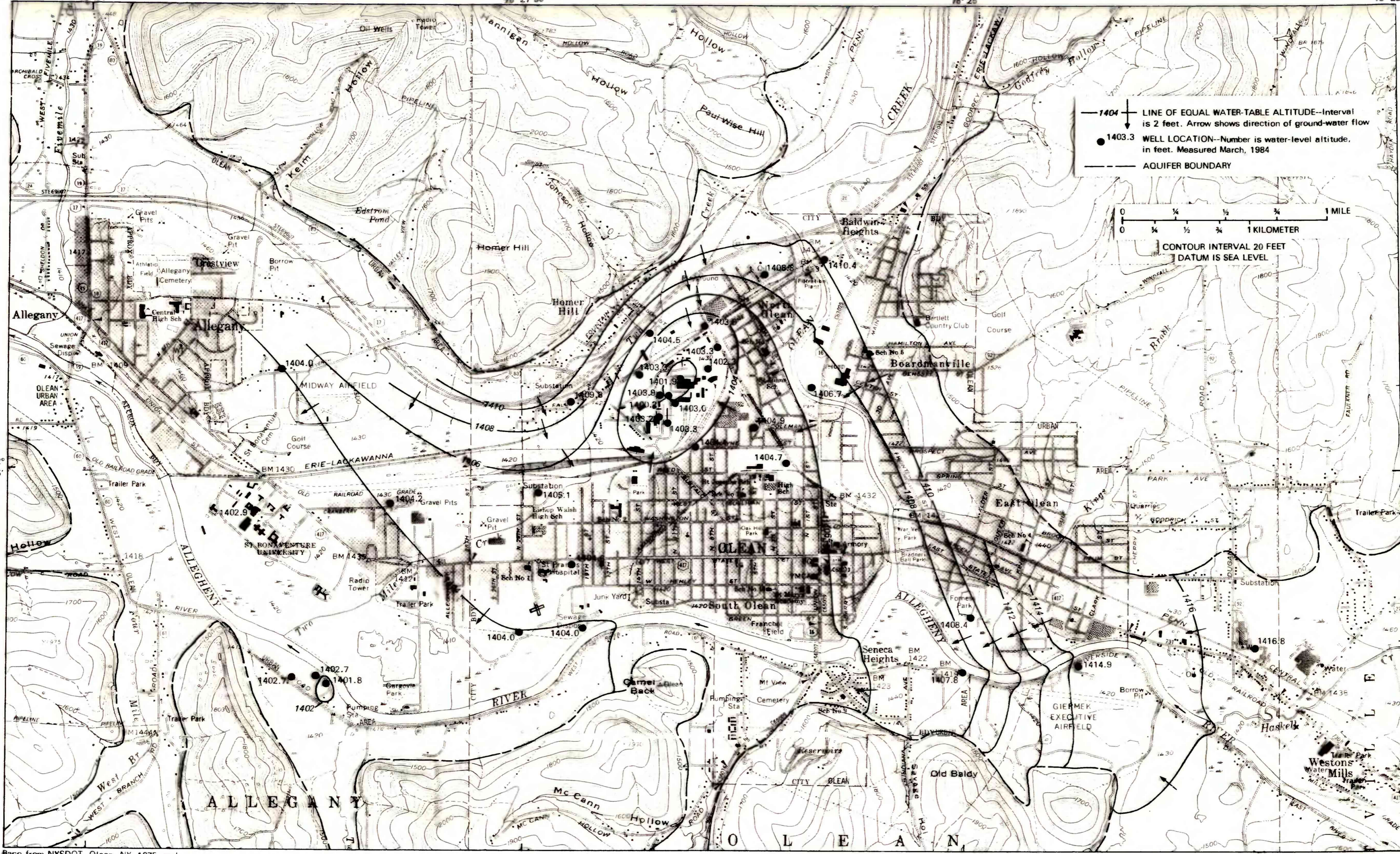
WATER-TABLE ALTITUDE AND DIRECTION OF GROUND-WATER FLOW AT OLEAN, MARCH 20-21, 1984
