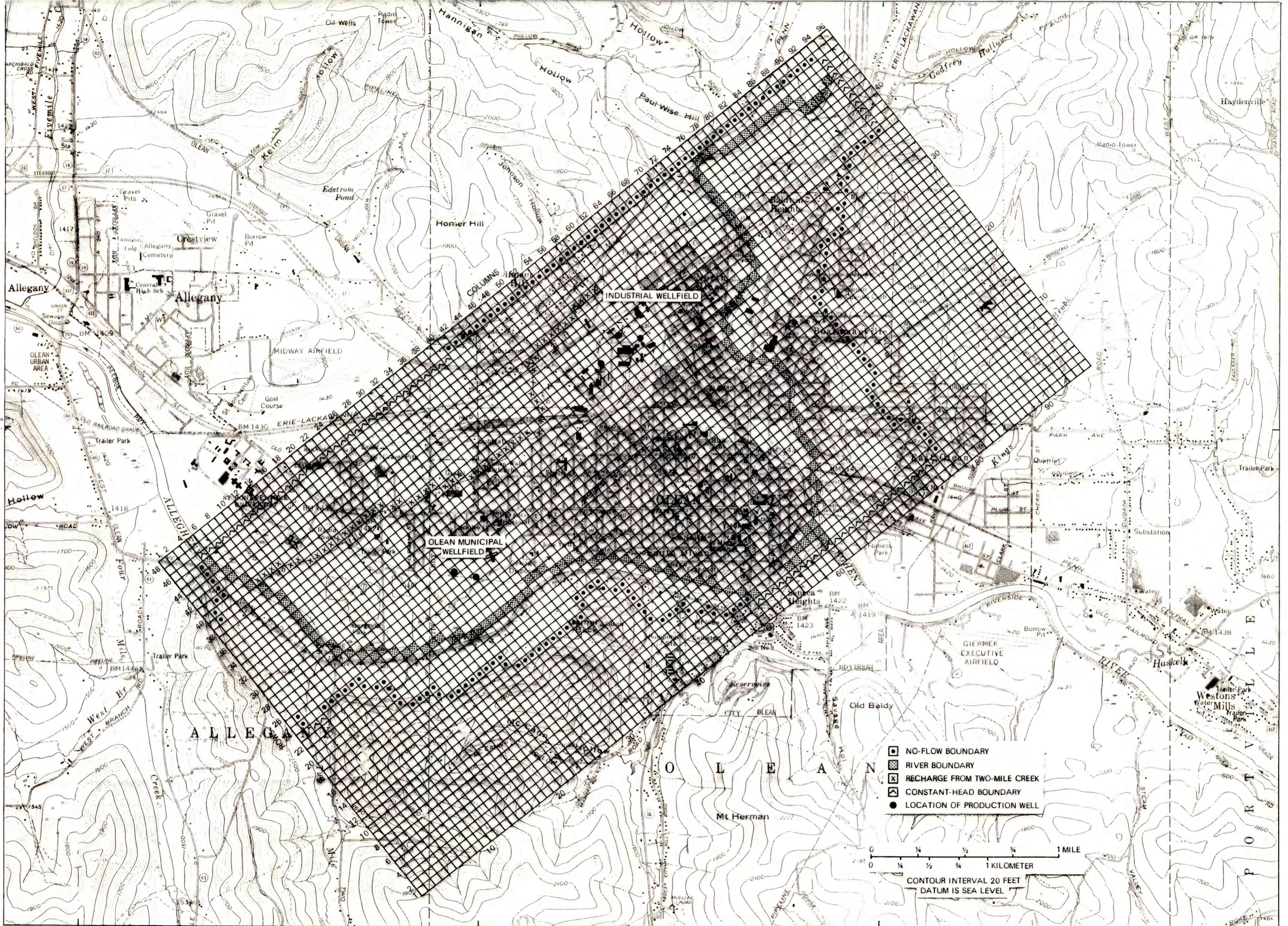
FINITE-DIFFERENCE GRID AND BOUNDARY CONDITIONS USED IN SOLUTE-TRANSPORT MODEL
