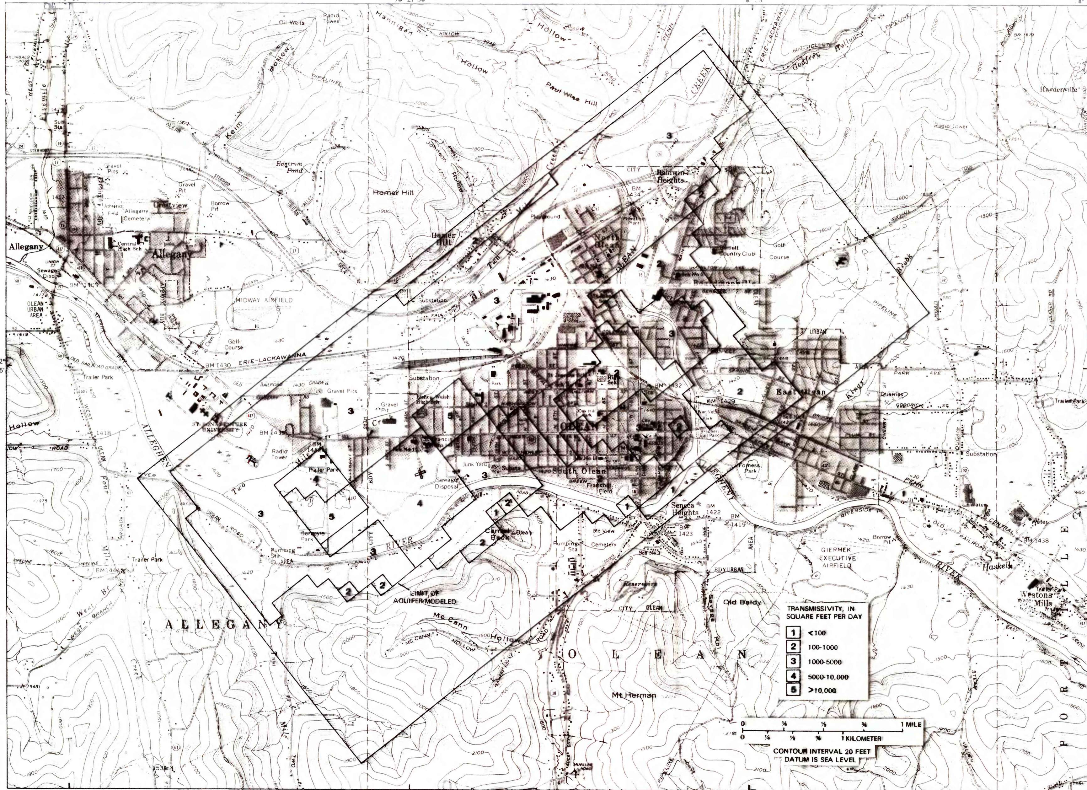
TRANSMISSIVITY OF OUTWASH AQUIFER USED IN SOLUTE-TRANSPORT MODEL
