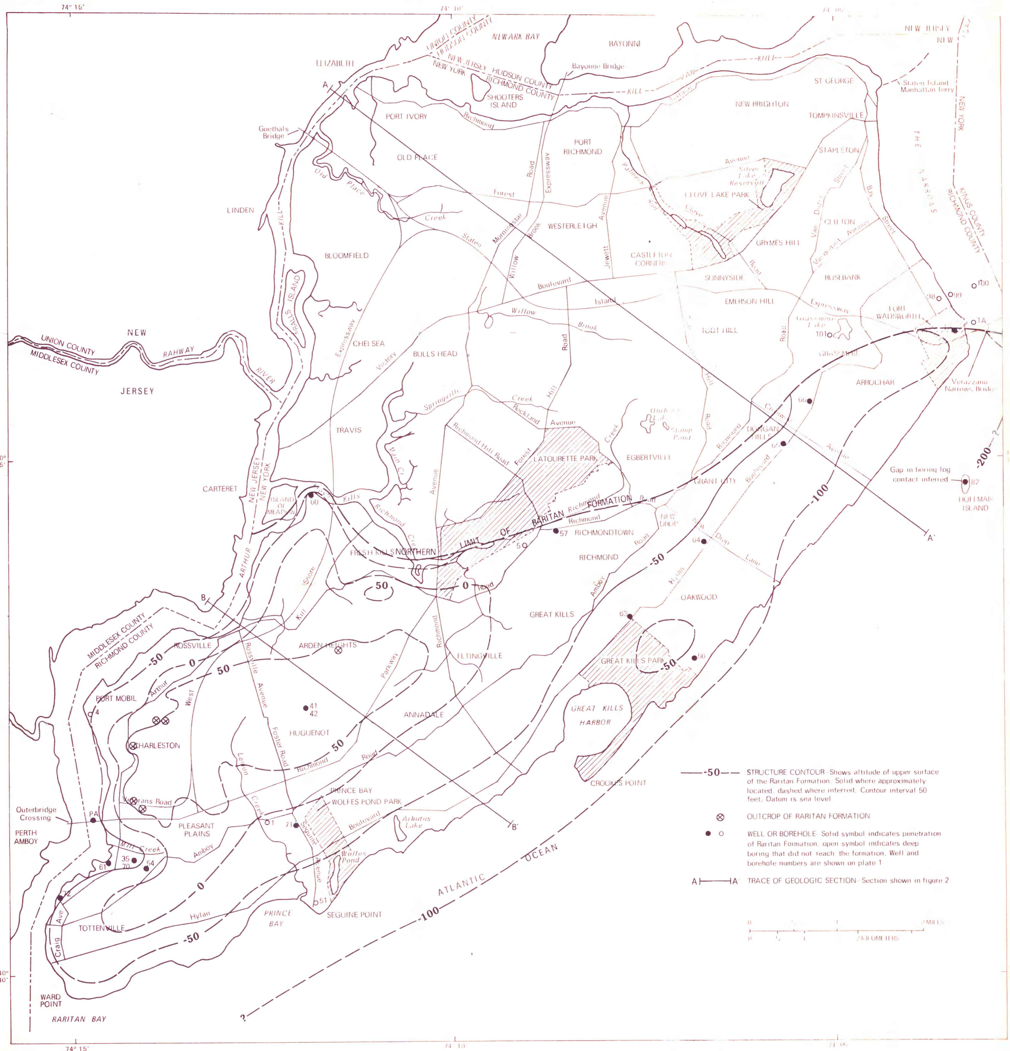
PLATE 3 CONFIGURATION OF THE SURFACE OF THE RARITAN FORMATION ON STATEN ISLAND
