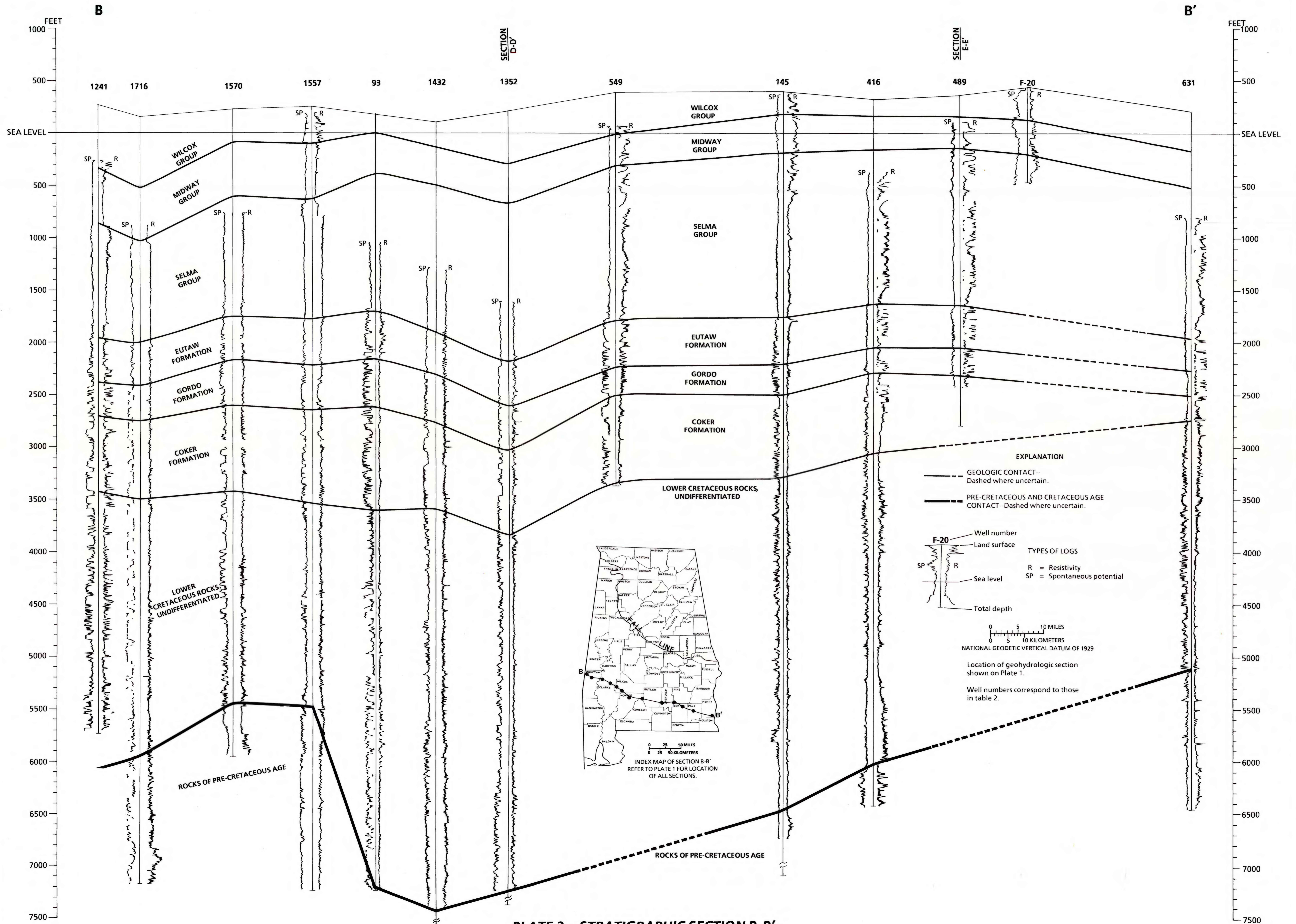
PLATE 3.--STRATIGRAPHIC SECTION B-B'
