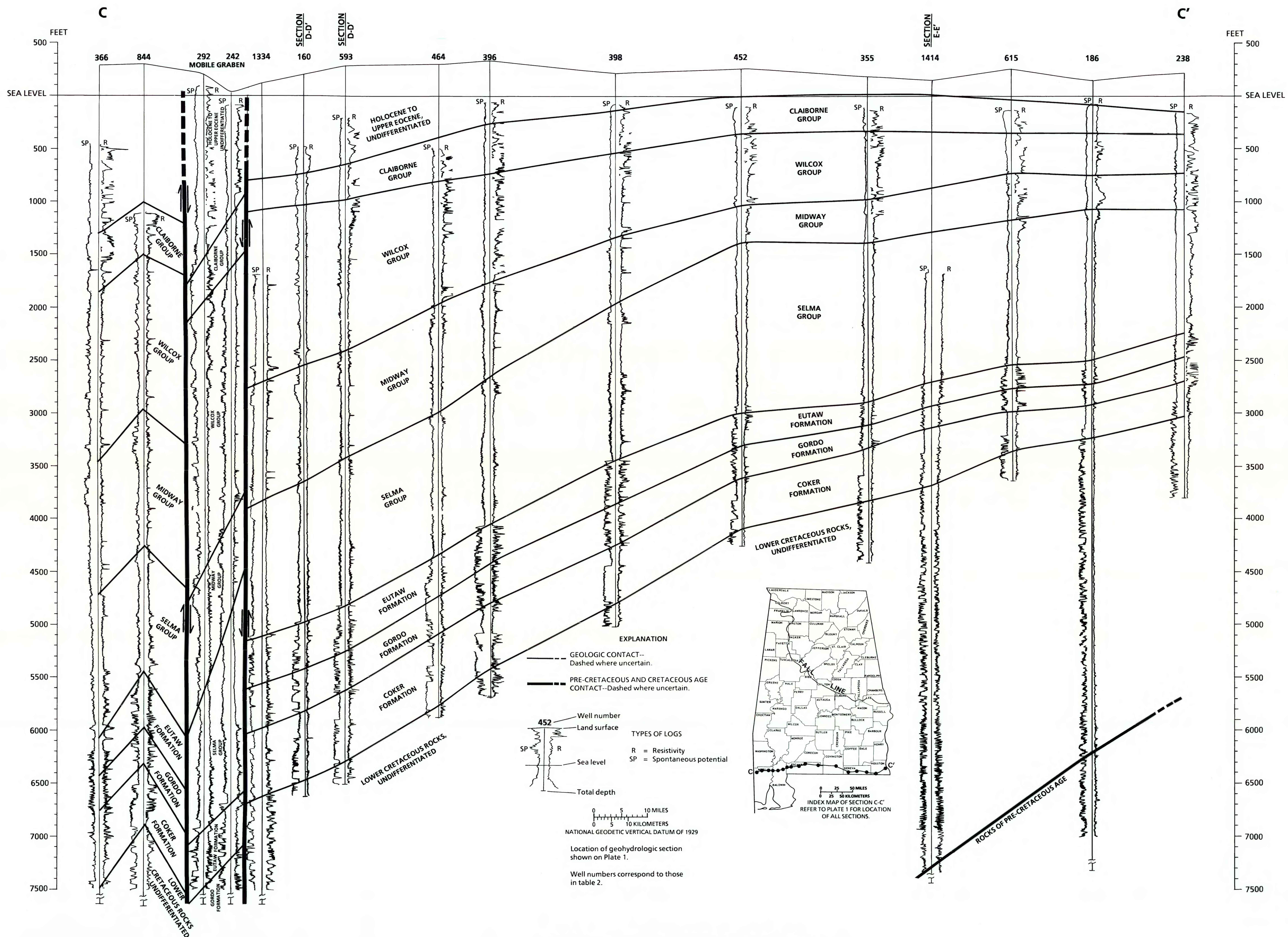
PLATE 4.--STRATIGRAPHIC SECTION C-C'
