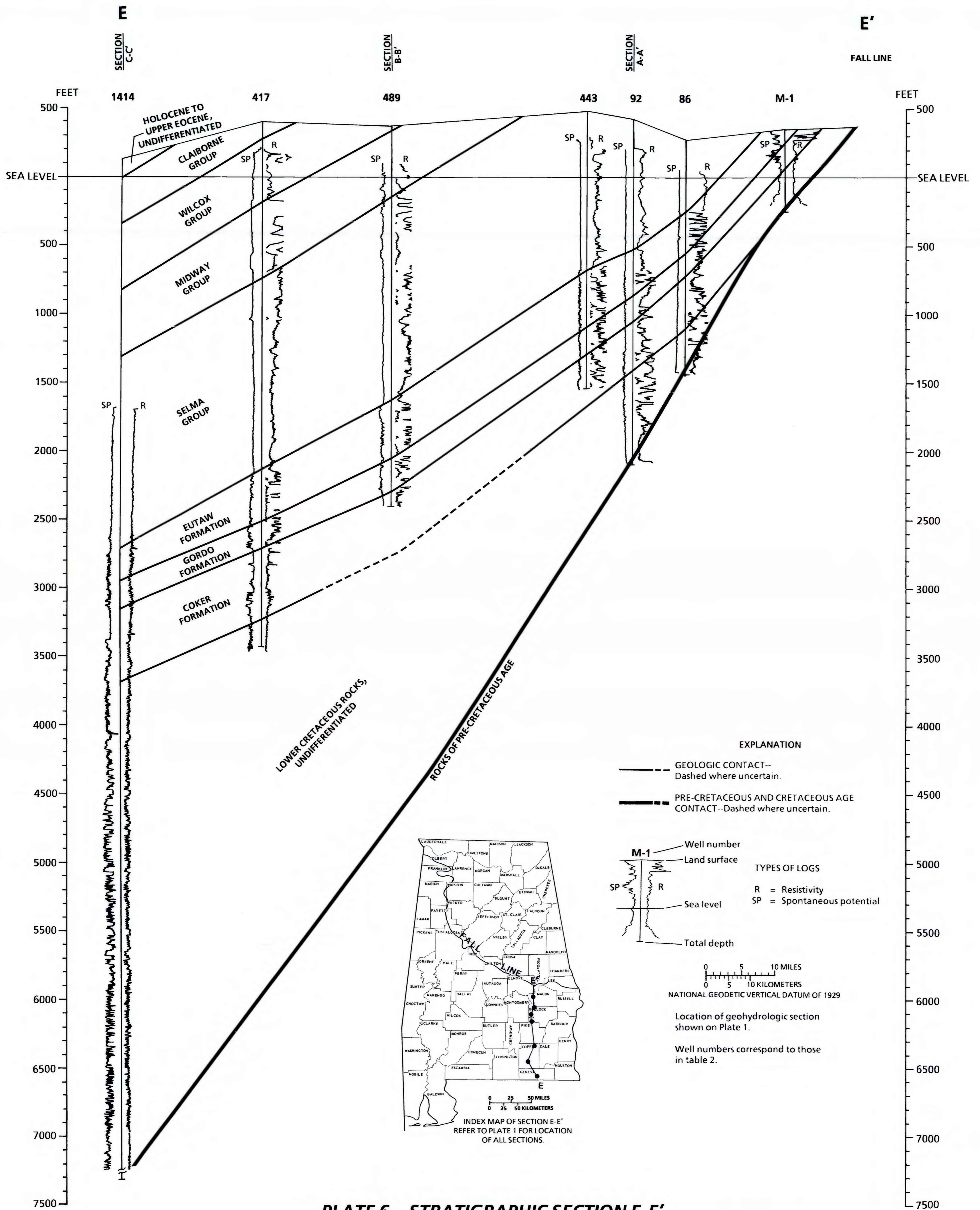
PLATE 6.--STRATIGRAPHIC SECTION E-E'
