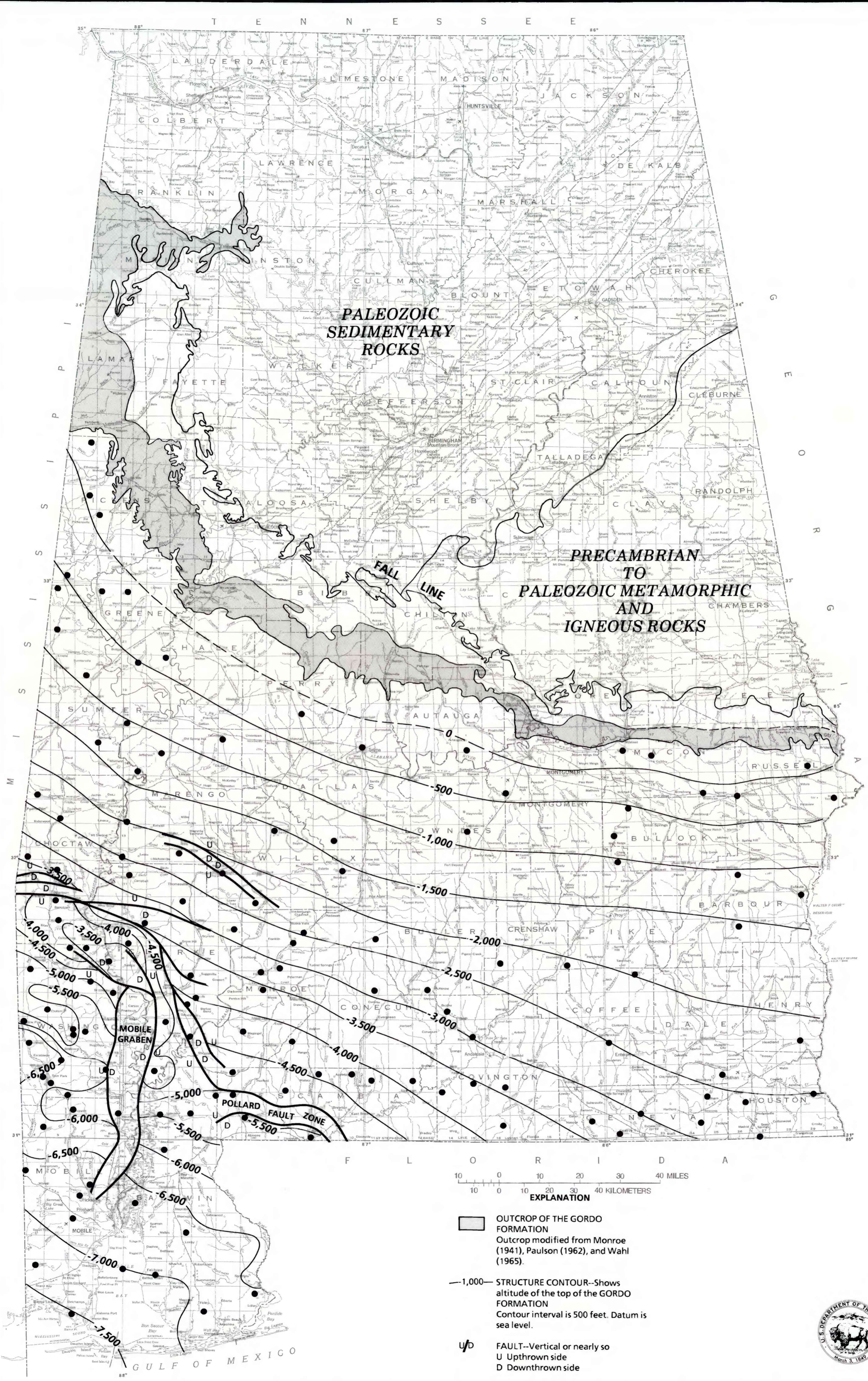
PLATE 10.--CONFIGURATION OF TOP OF THE GORDO FORMATION
