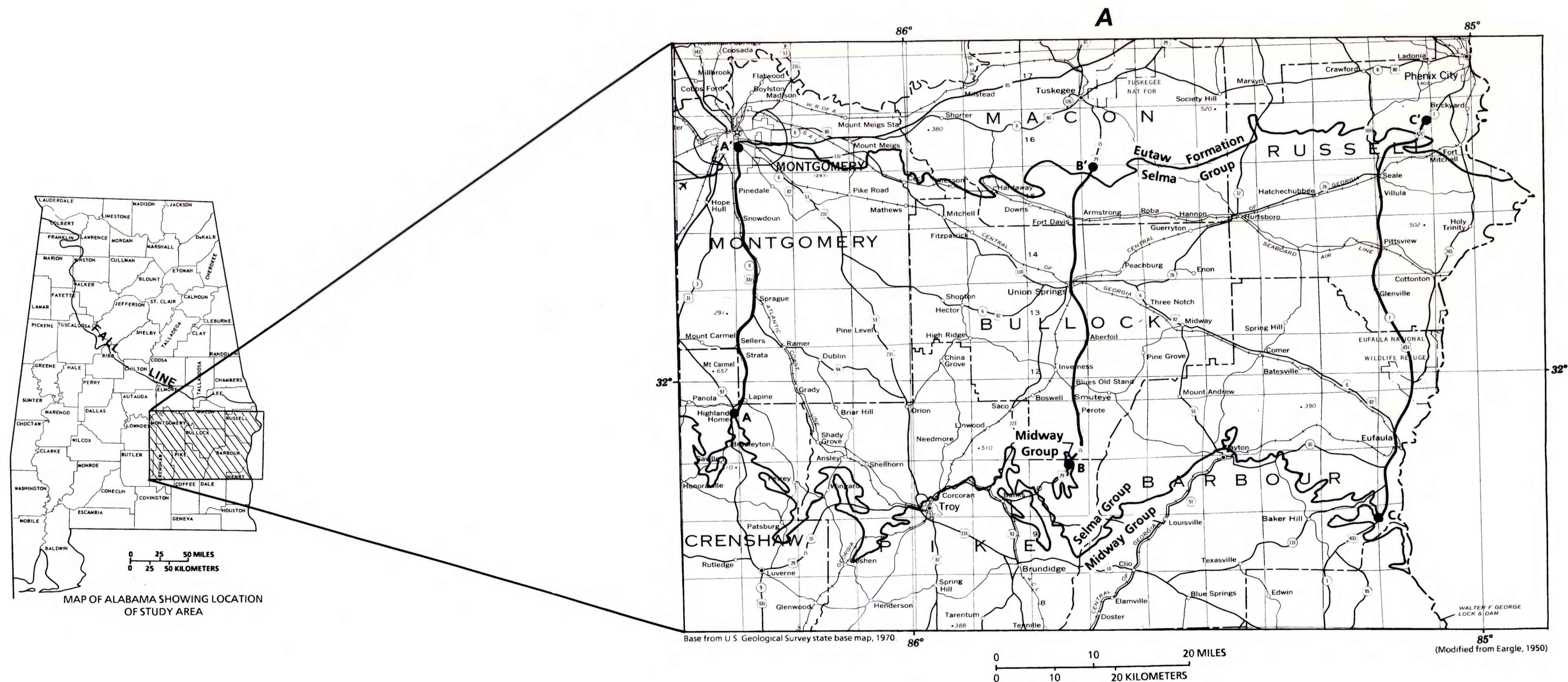
PLATE 17.--GENERALIZED OUTCROP OF THE SELMA GROUP IN THE NORTHEASTERN PART OF THE COASTAL PLAIN IN ALABAMA AND LINES OF MEASURED GEOLOGIC PROFILES. A, MAP SHOWING OUTCROP OF THE SELMA GROUP AND LINES OF MEASURED GEOLOGIC PROFILES (A-A', B-B', and C-C'). B, LITHOLOGIC COLUMNS FROM MEASURED PROFILES SHOWING CORRELATION AND FACIES CHANGES IN THE OUTCROPPING FORMATIONS OF THE SELMA GROUP.
