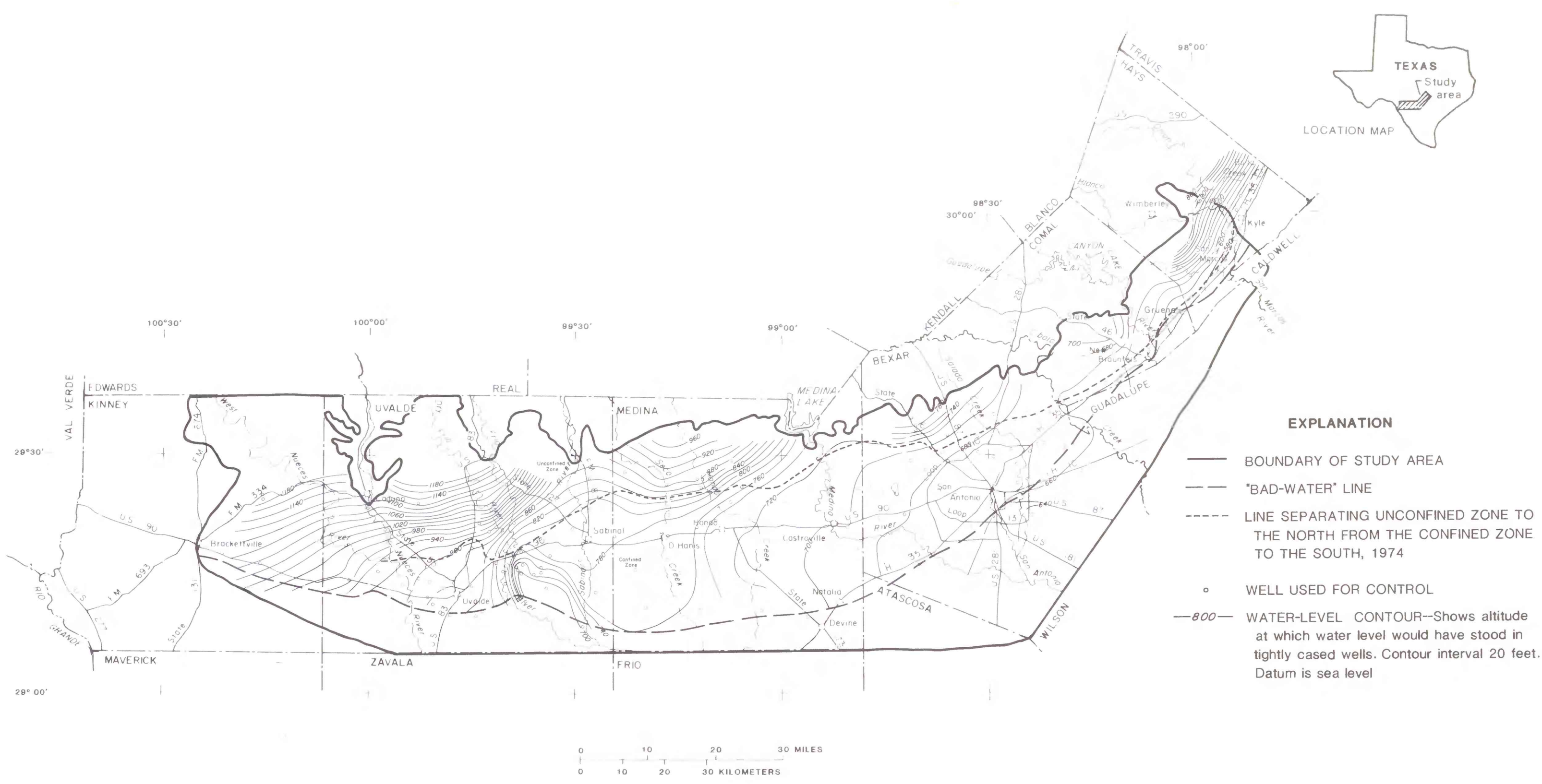
Figure 5.--Water levels in the Edwards aquifer, July 1974
