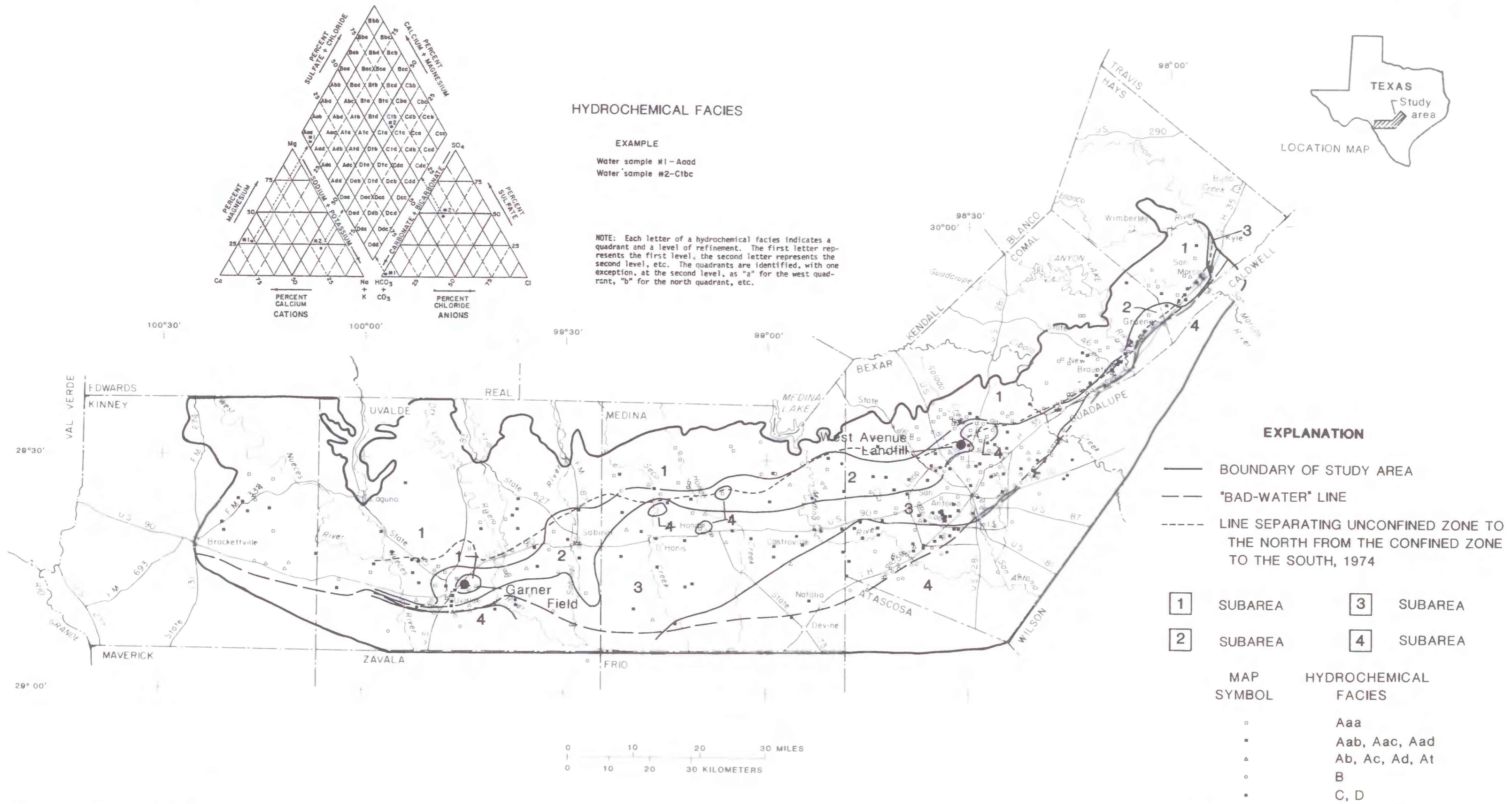
Figure 11.--Hydrochemical facies.
