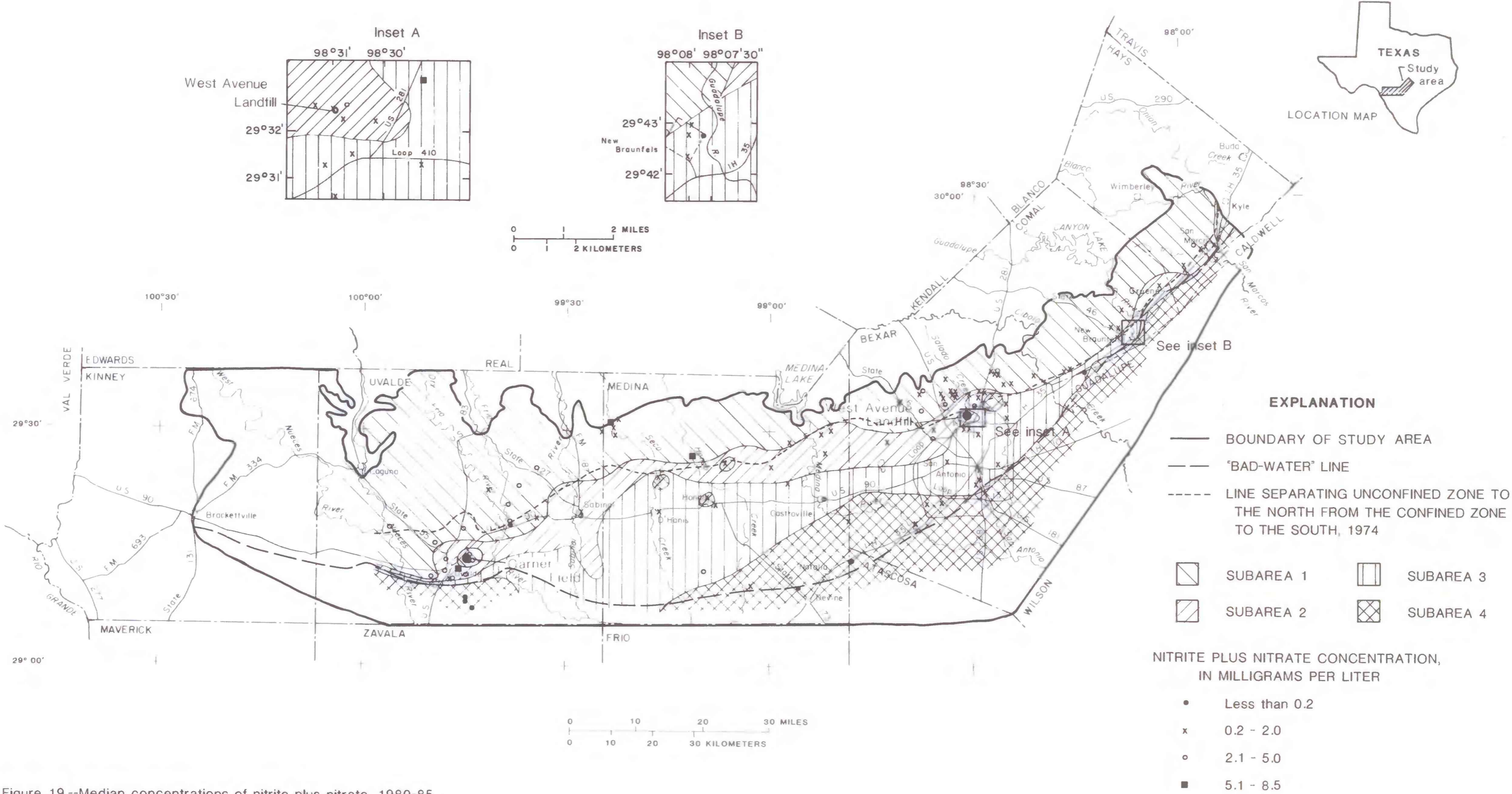
Figure 19.--Median concentrations of nitrite plus nitrate, 1980-85.
