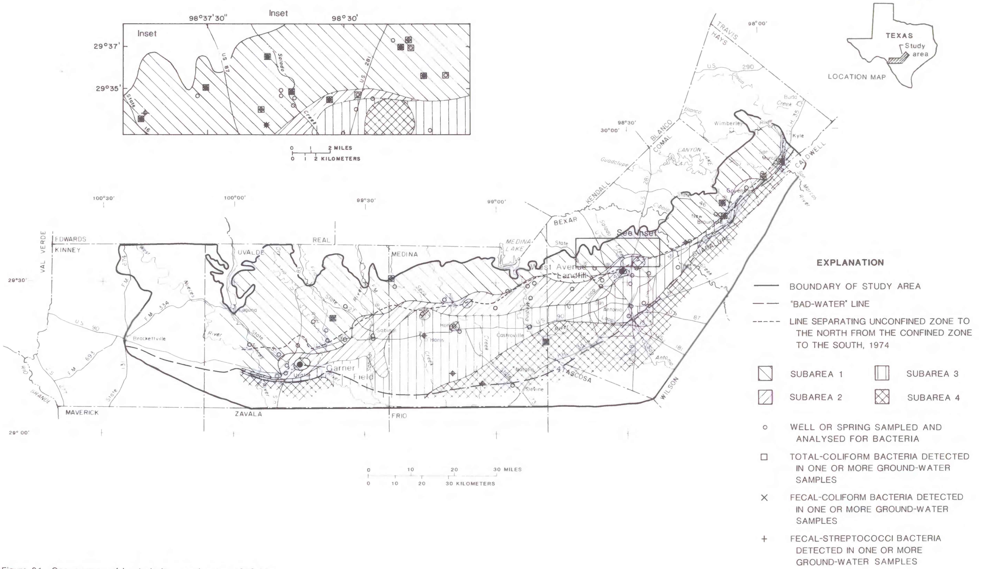
Figure 21.--Occurrences of bacteria in ground water, 1976-83.
