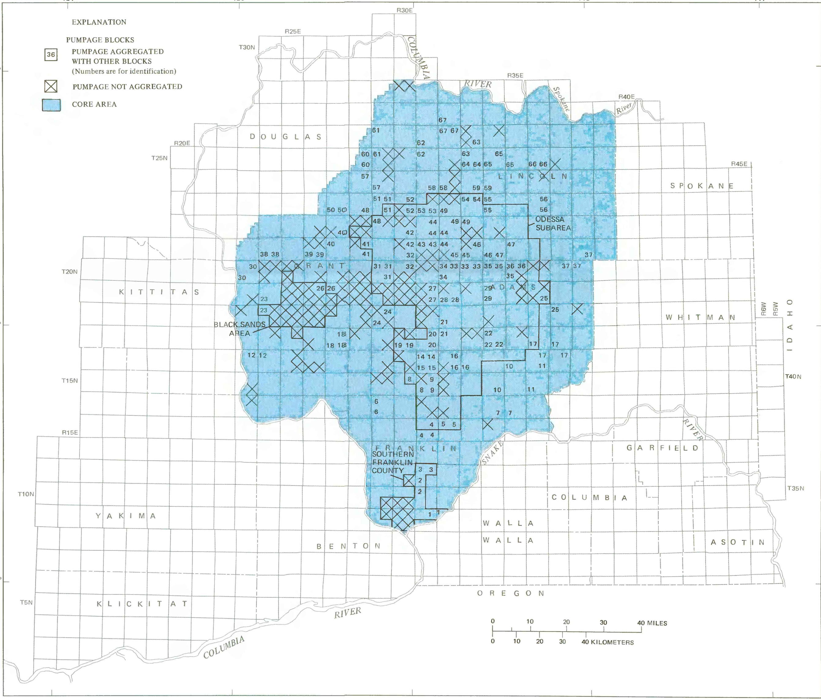
Figure F--Location of pumping centers and ground-water pumpage blocks, and aggregation of blocks in the core area, by quarter township.
