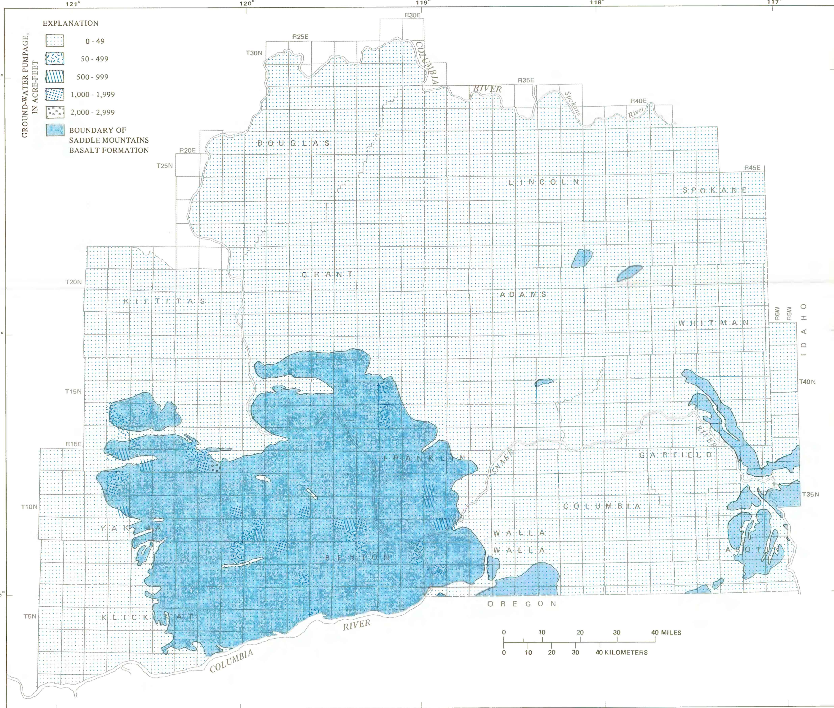
Figure D--Pumpage from the Saddle Mountains Unit in the Columbia Plateau, Washington, by quarter township, 1984.
