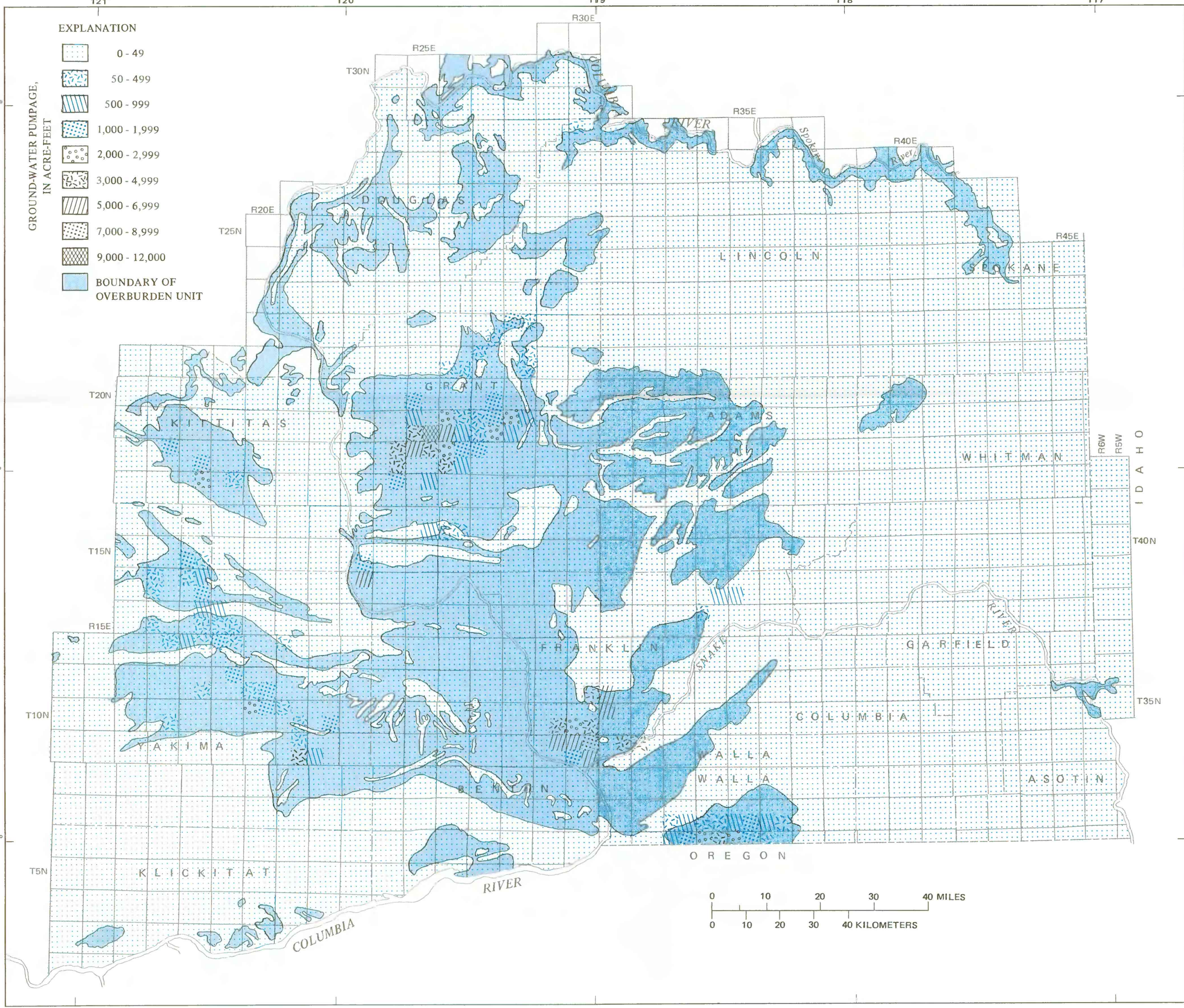
Figure E--Pumpage from the Overburden Unit in the Columbia Plateau, Washington, by quarter township, 1984.
