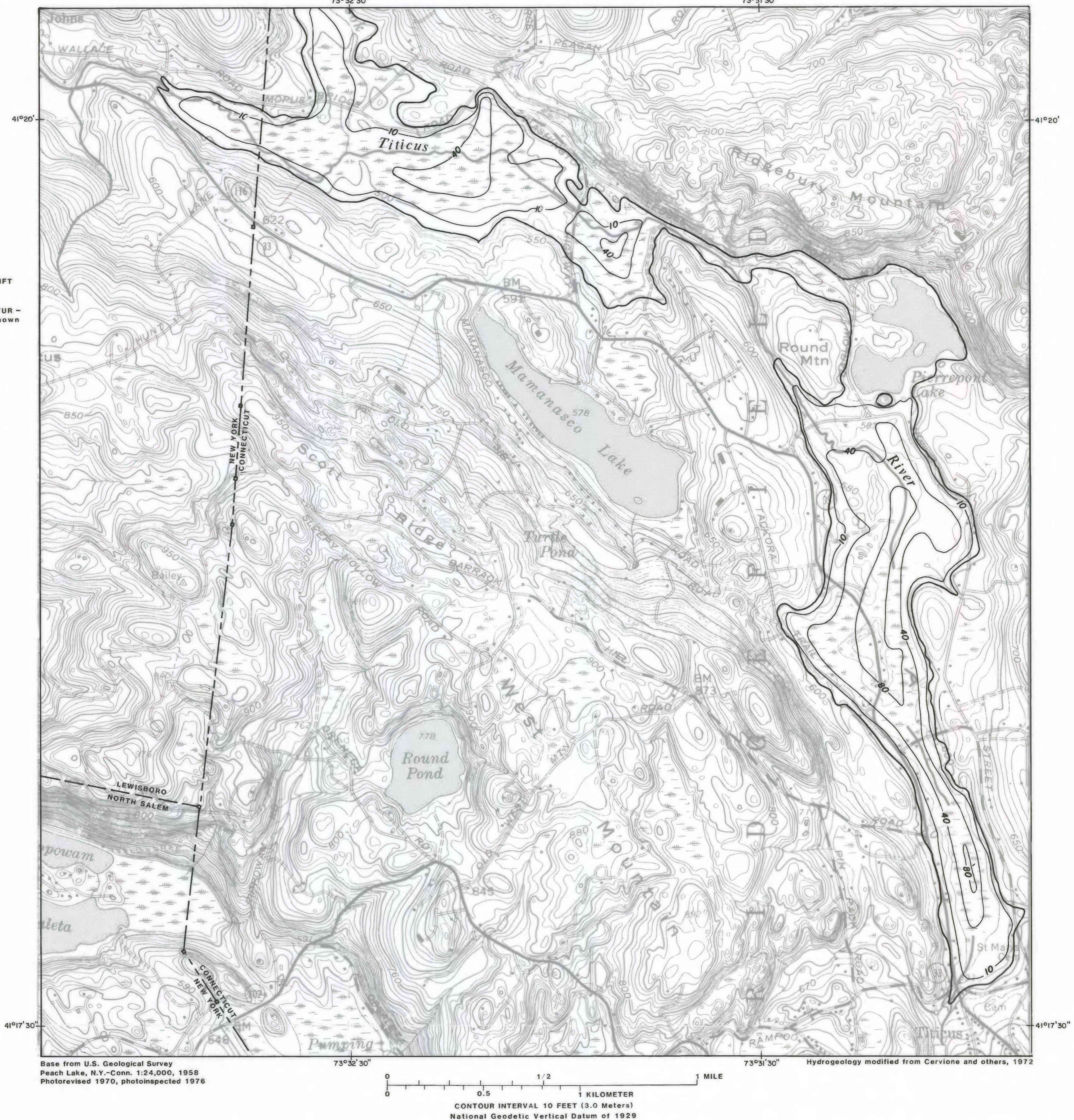
SATURATED THICKNESS OF THE STRATIFIED-DRIFT AQUIFER IN THE TITICUS RIVER VALLEY, RIDGEFIELD, CONNECTICUT
