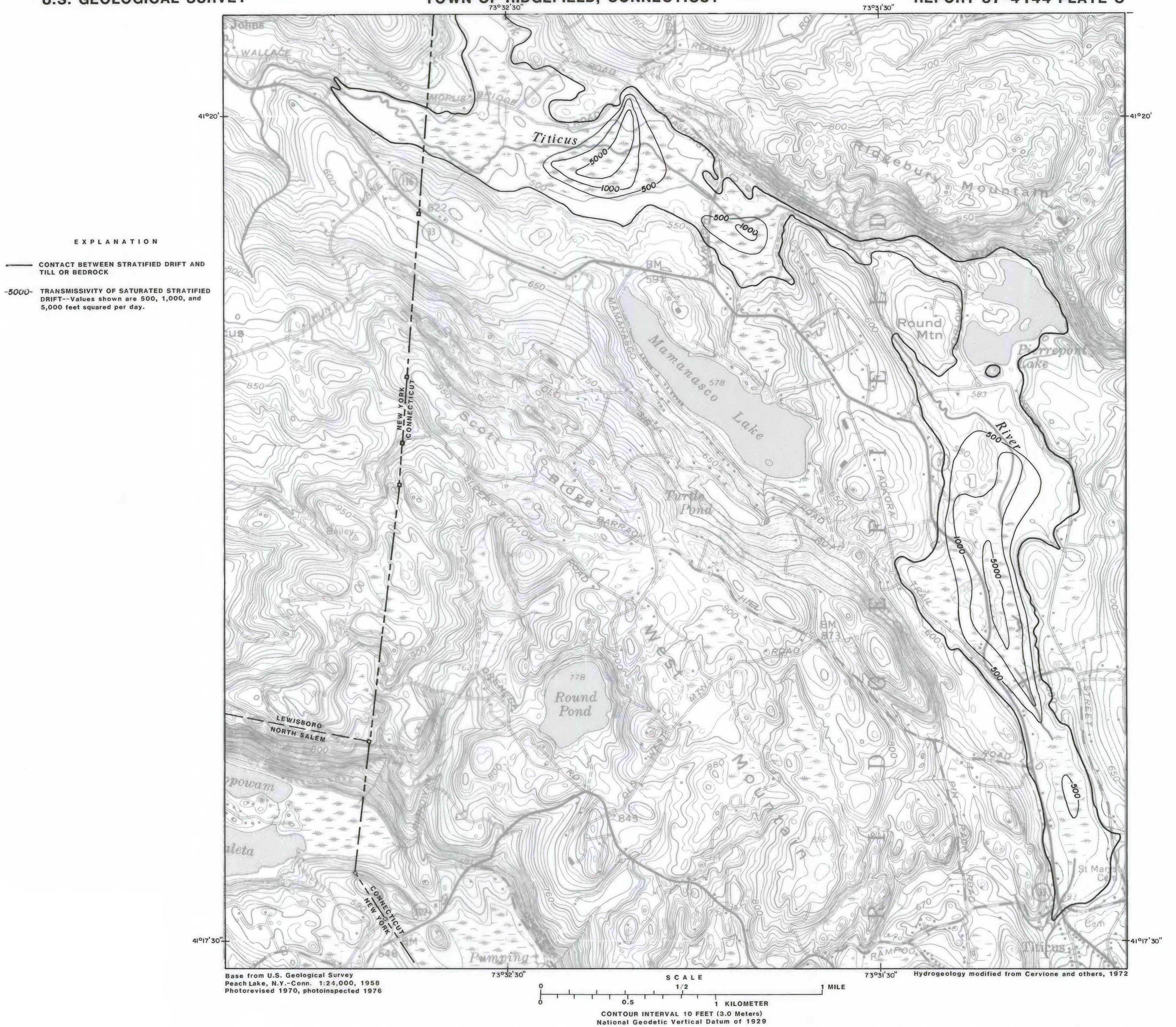
TRANSMISSIVITY OF THE STRATIFIED-DRIFT AQUIFER IN THE TITICUS RIVER VALLEY, RIDGEFIELD, CONNECTICUT
