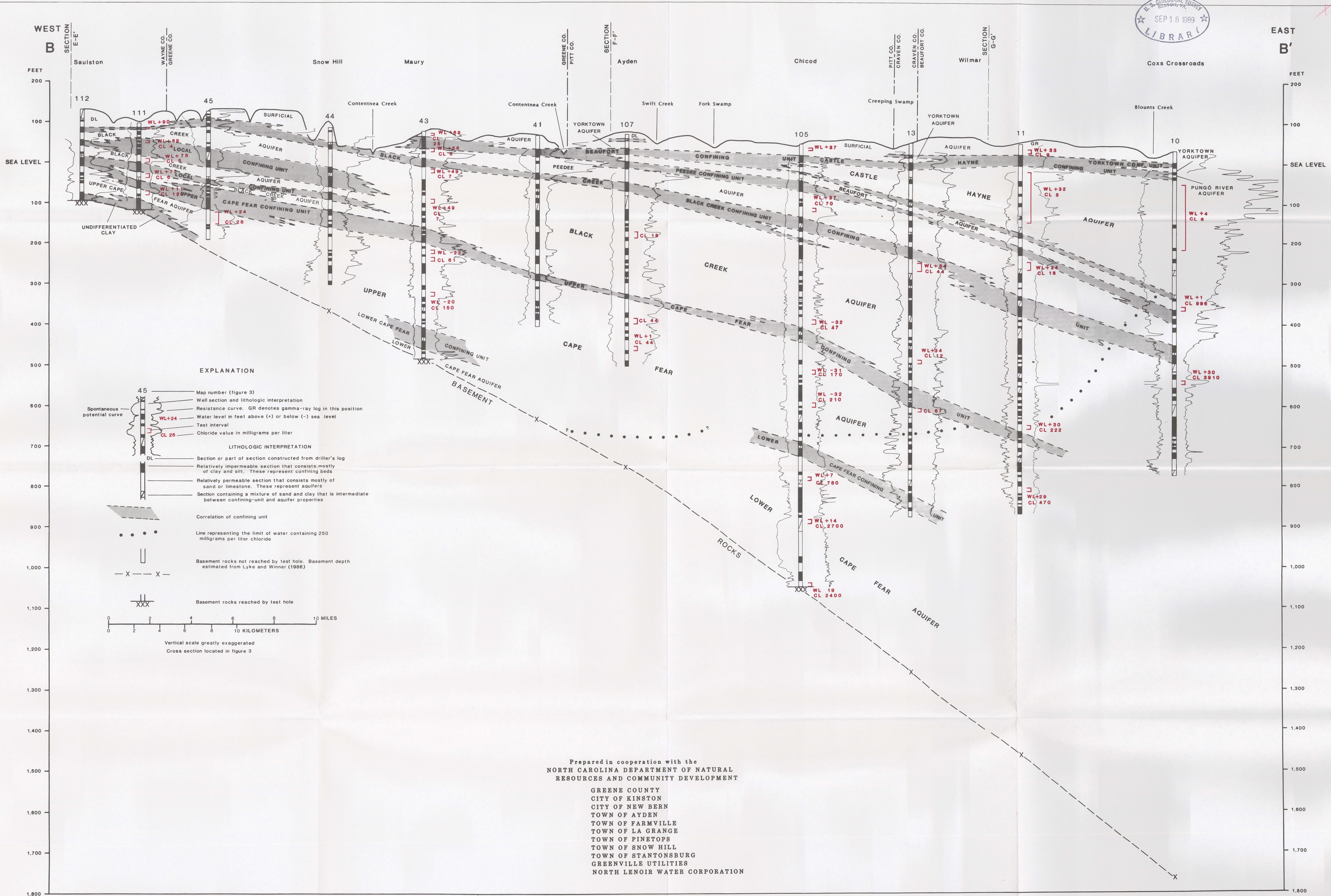
HYDROGEOLOGIC SECTION B-B' FROM SAULSTON, WAYNE COUNTY TO COX'S CROSSROADS, BEAUFORT COUNTY
