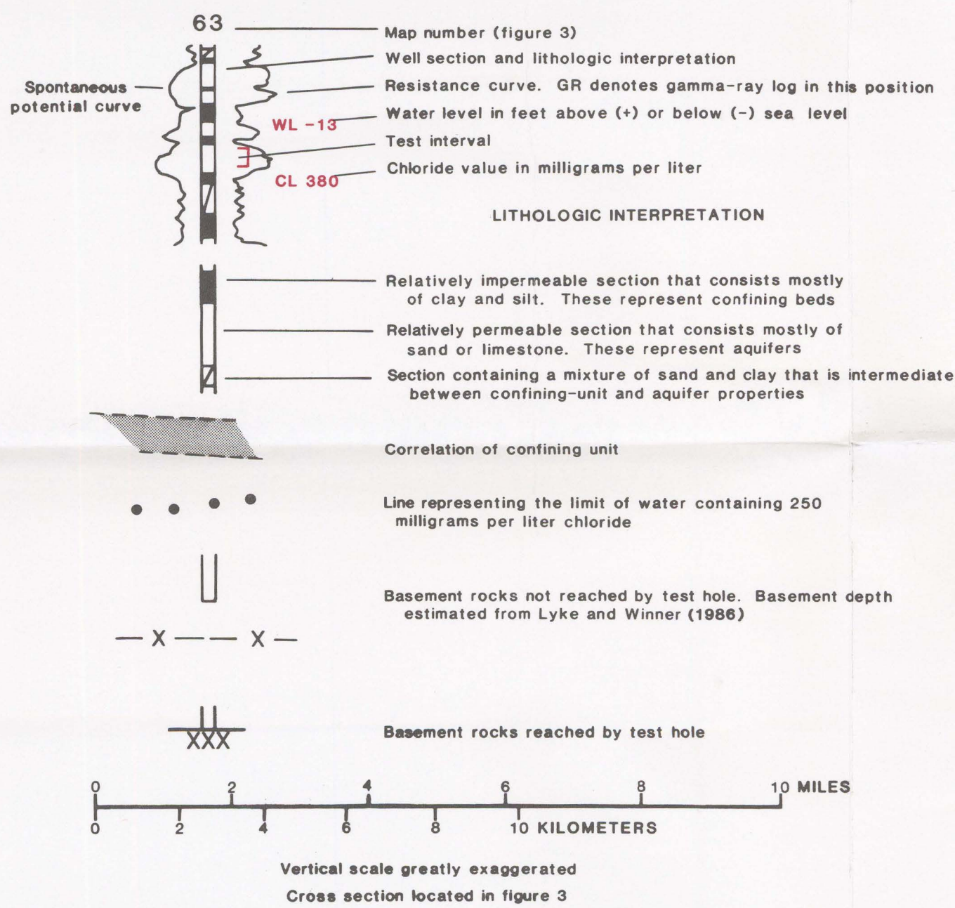
HYDROGEOLOGIC SECTION C-C' FROM INSTITUTE, LENOIR COUNTY TO FORT BARNWELL, CRAVEN COUNTY
