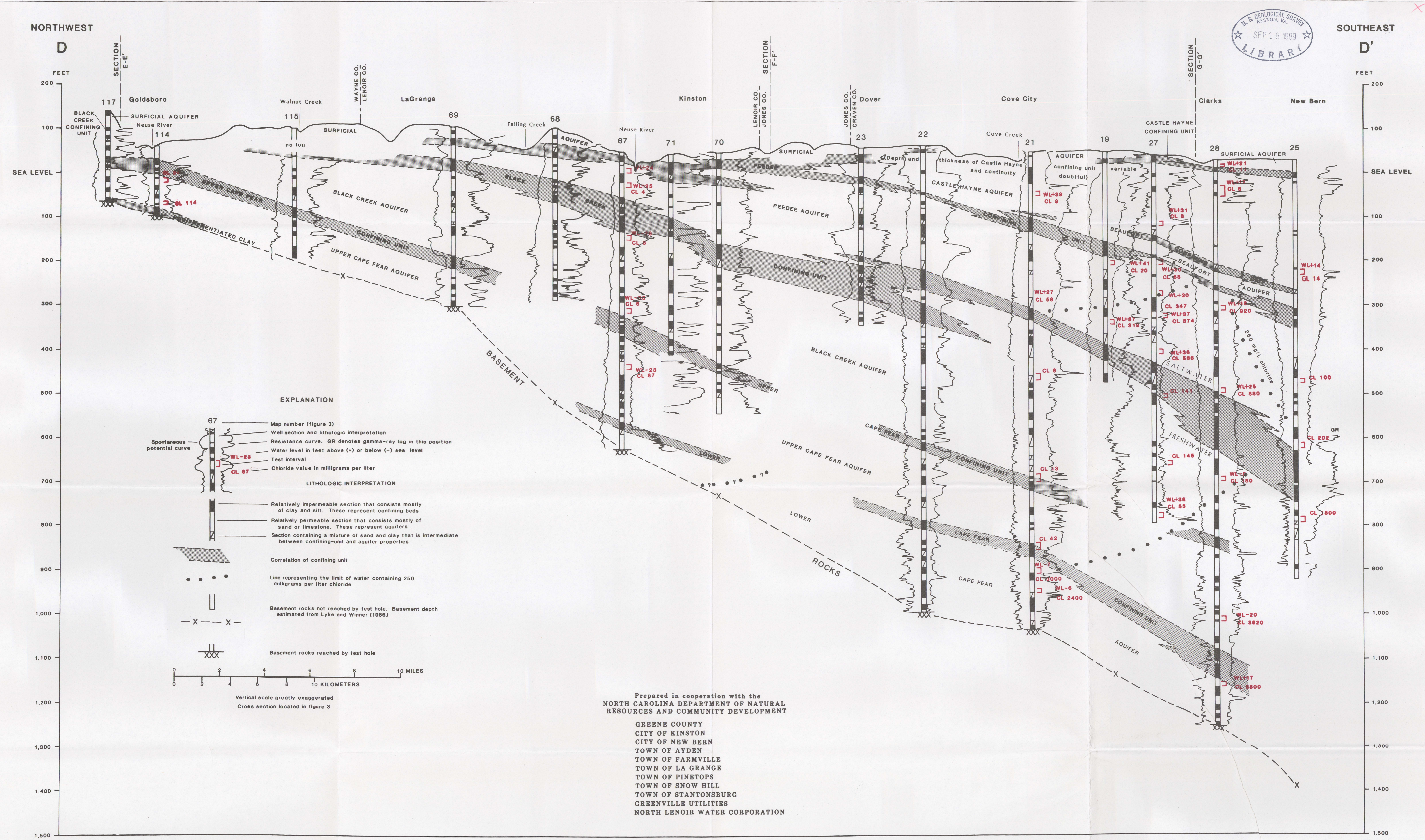
HYDROGEOLOGIC SECTION D-D' FROM GOLDSBORO, WAYNE COUNTY TO NEW BERN, CRAVEN COUNTY
