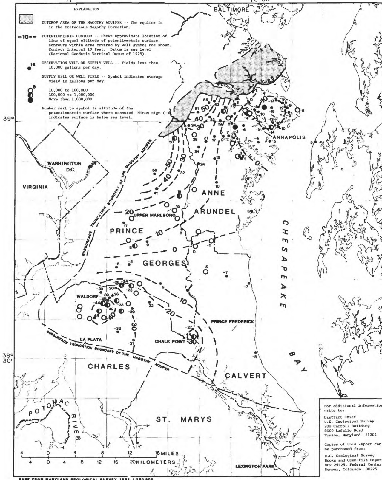
POTENTIOMETRIC SURFACE OF THE MAGOTHY AQUIFER IN SOUTHERN MARYLAND DURING FALL OF 1986
