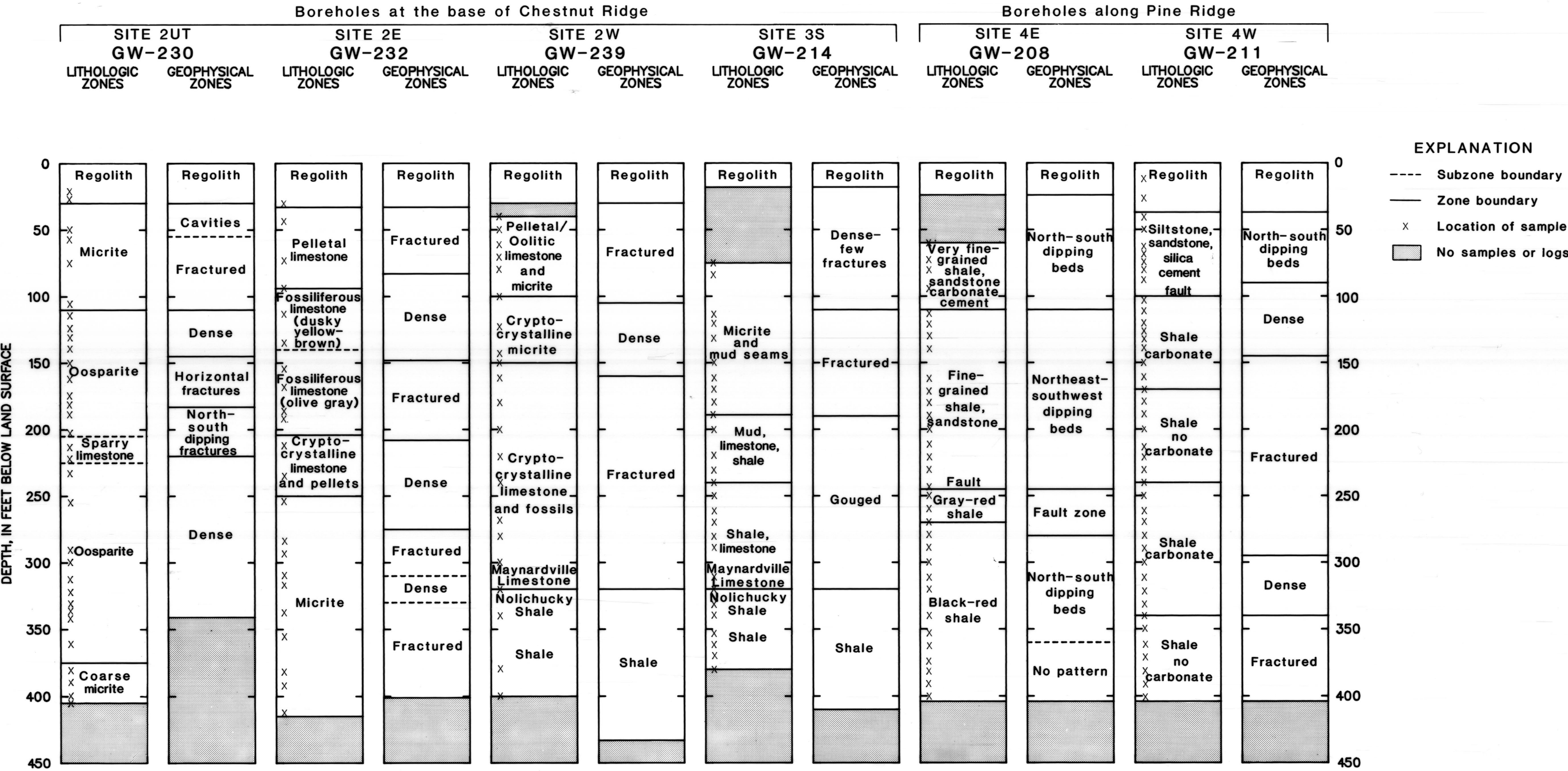
Plate 1.--Comparison of zones delineated from lithologic samples and from geophysical logs.
