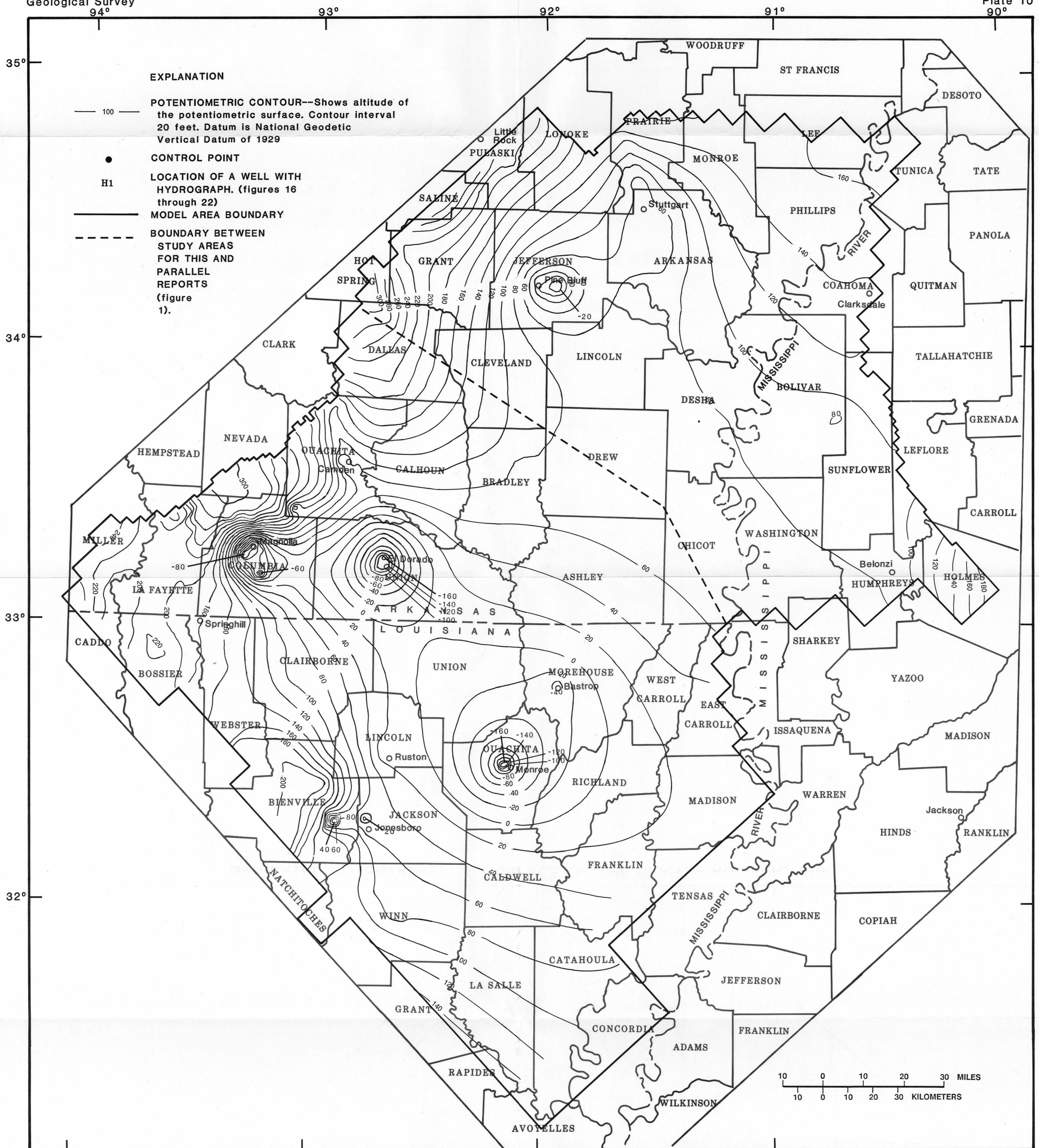
SIMULATED POTENTIOMETRIC SURFACE OF THE SPARTA AQUIFER, 1985
