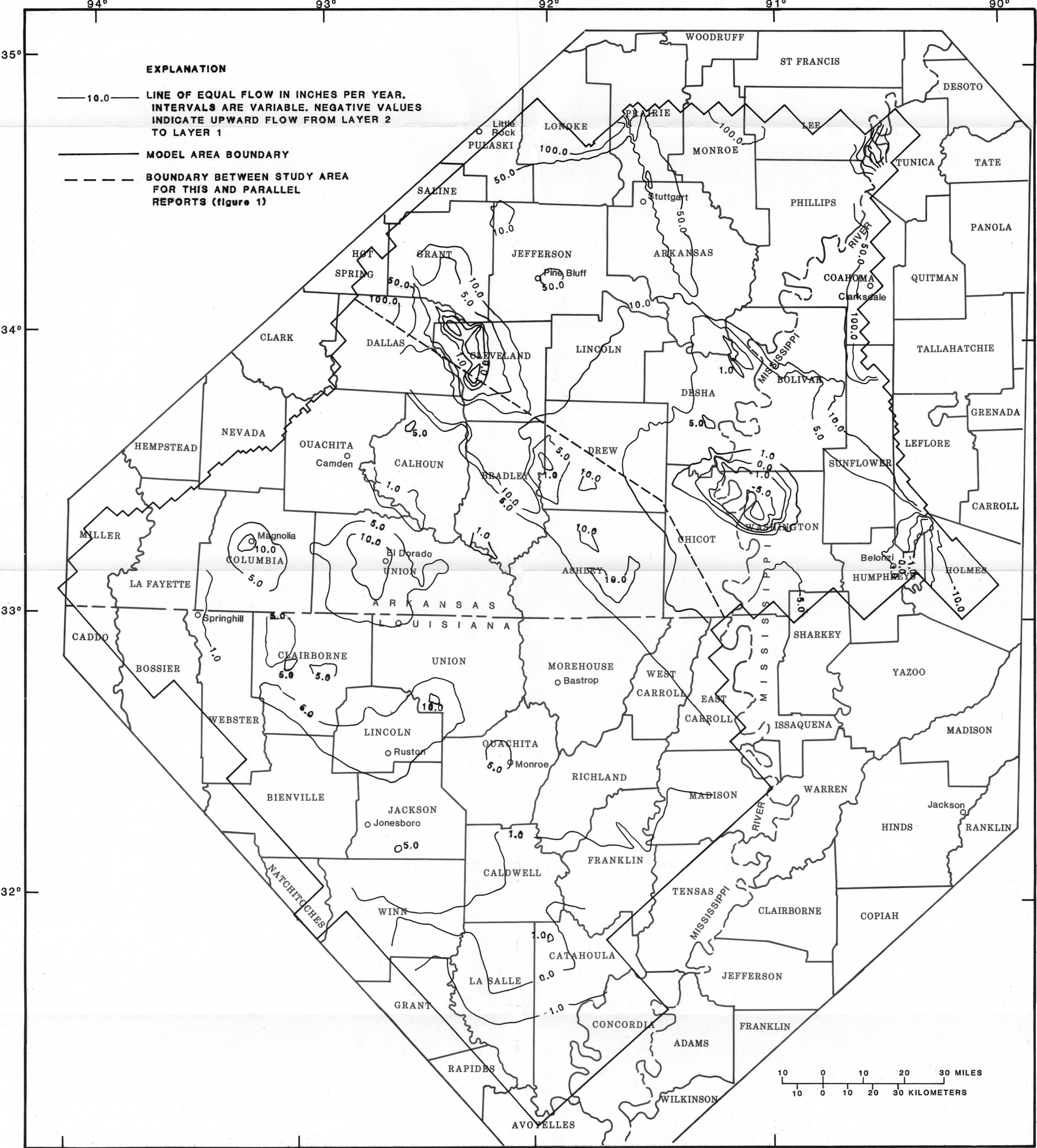
SIMULATED FLOW BETWEEN LAYERS 1 AND 2 IN 1985
