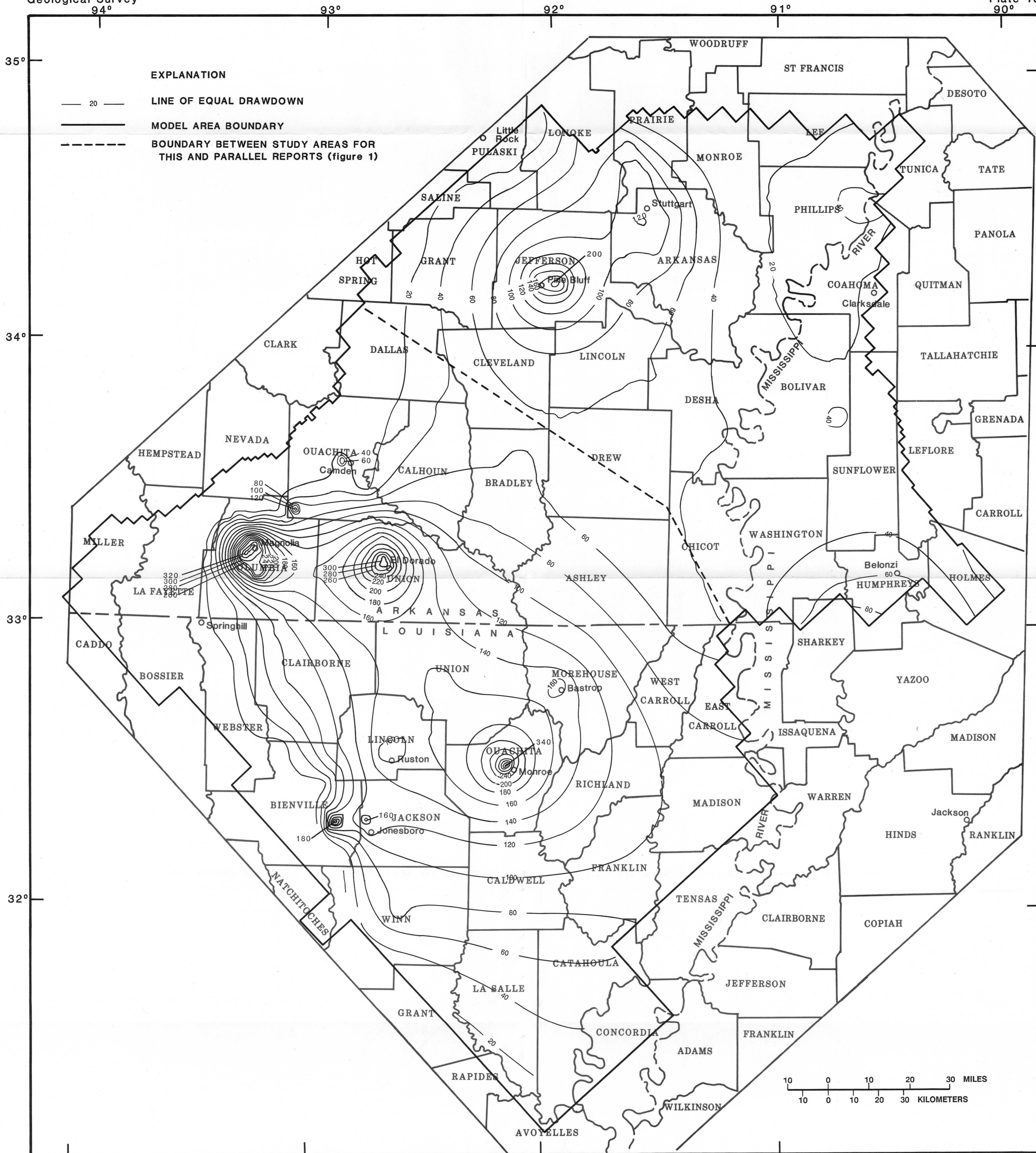
DRAWDOWN IN THE SPARTA AQUIFER BETWEEN PREDEVELOPMENT (1898) AND 1985
