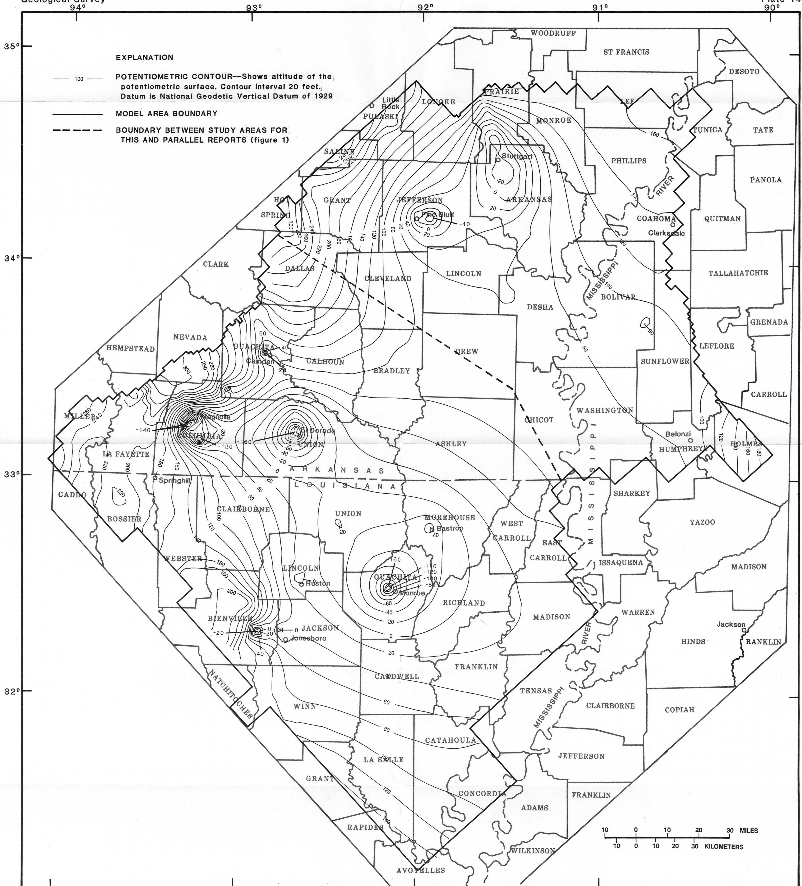
SIMULATED POTENTIOMETRIC SURFACE OF THE SPARTA AQUIFER IN 2005 WITH PUMPAGE IN THE GRAND PRAIRIE AREA DOUBLE 1985 VALUES
