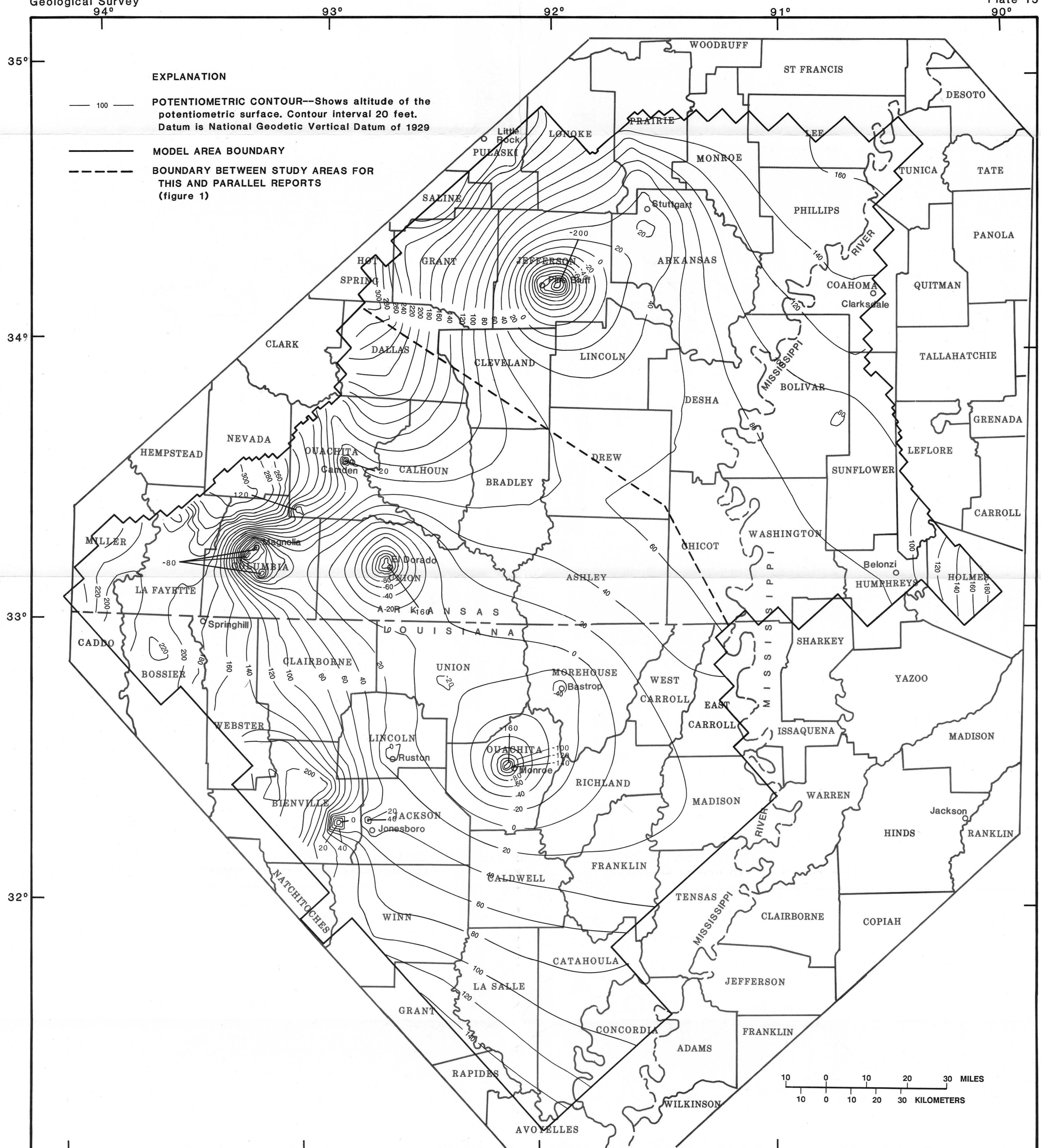
SIMULATED POTENTIOMETRIC SURFACE OF THE SPARTA AQUIFER IN 2005 WITH PUMPAGE IN THE PINE BLUFF AREA DOUBLE 1985 VALUES
