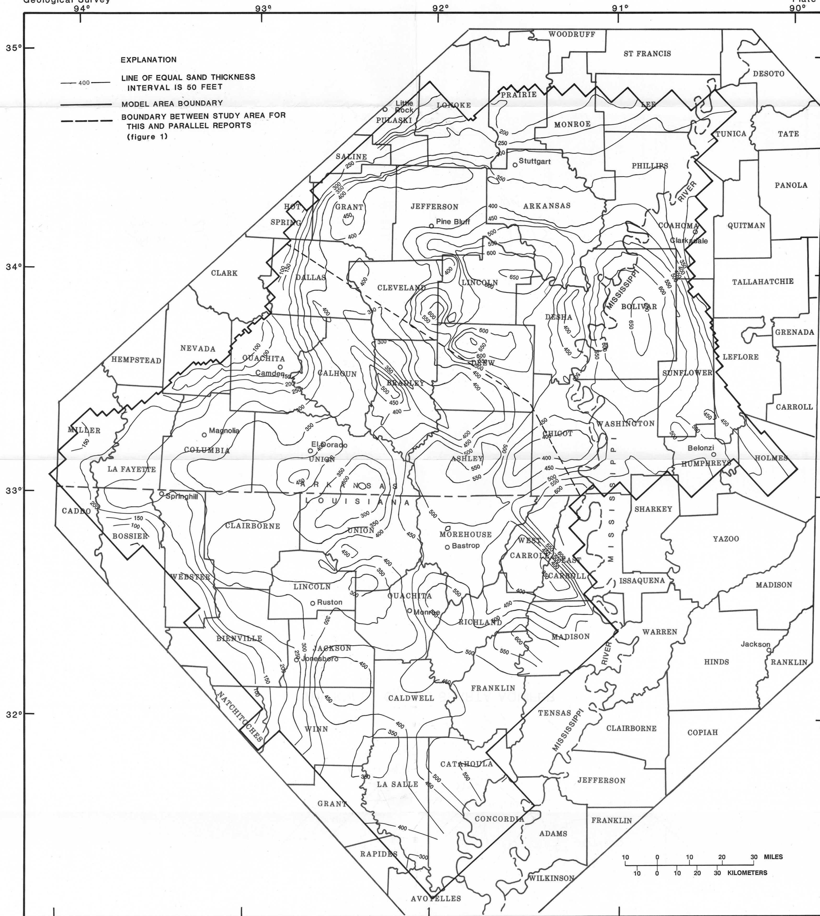
THICKNESS OF THE SPARTA AQUIFER
