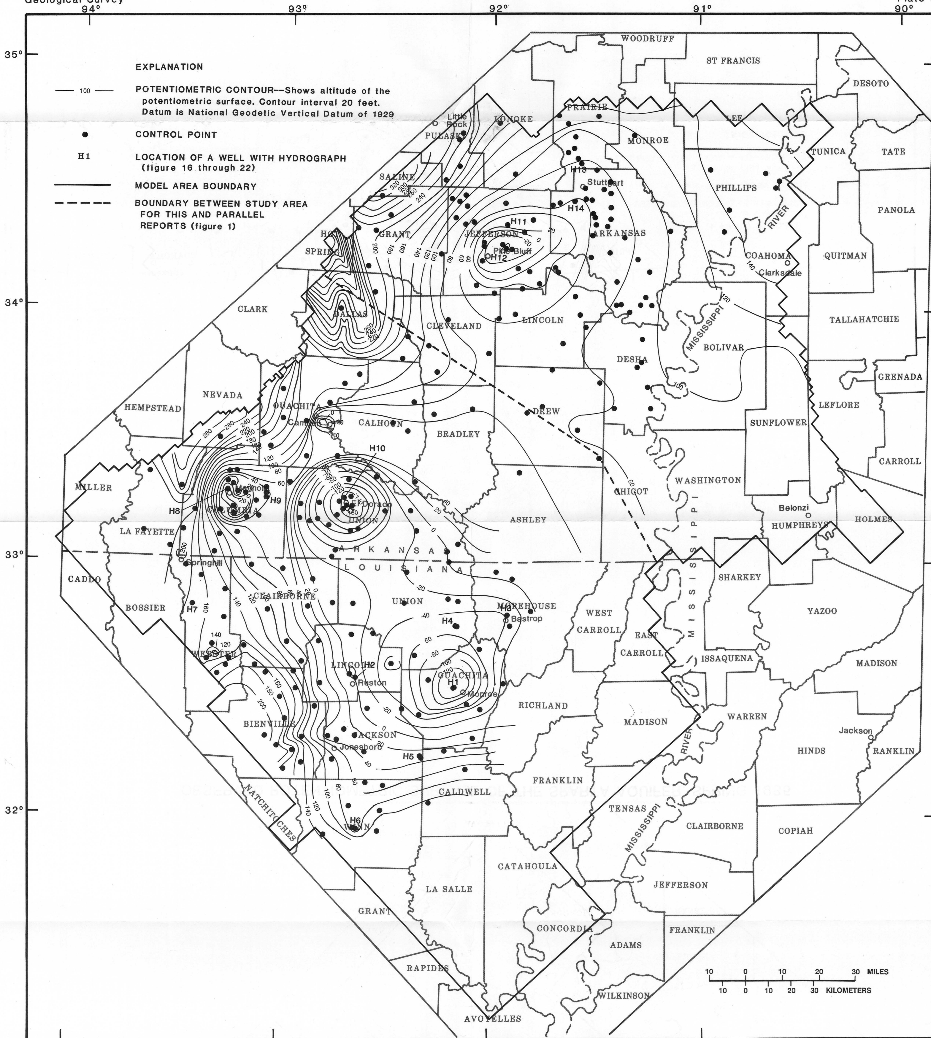
OBSERVED POTENTIOMETRIC SURFACE OF THE SPARTA AQUIFER, SPRING 1985
