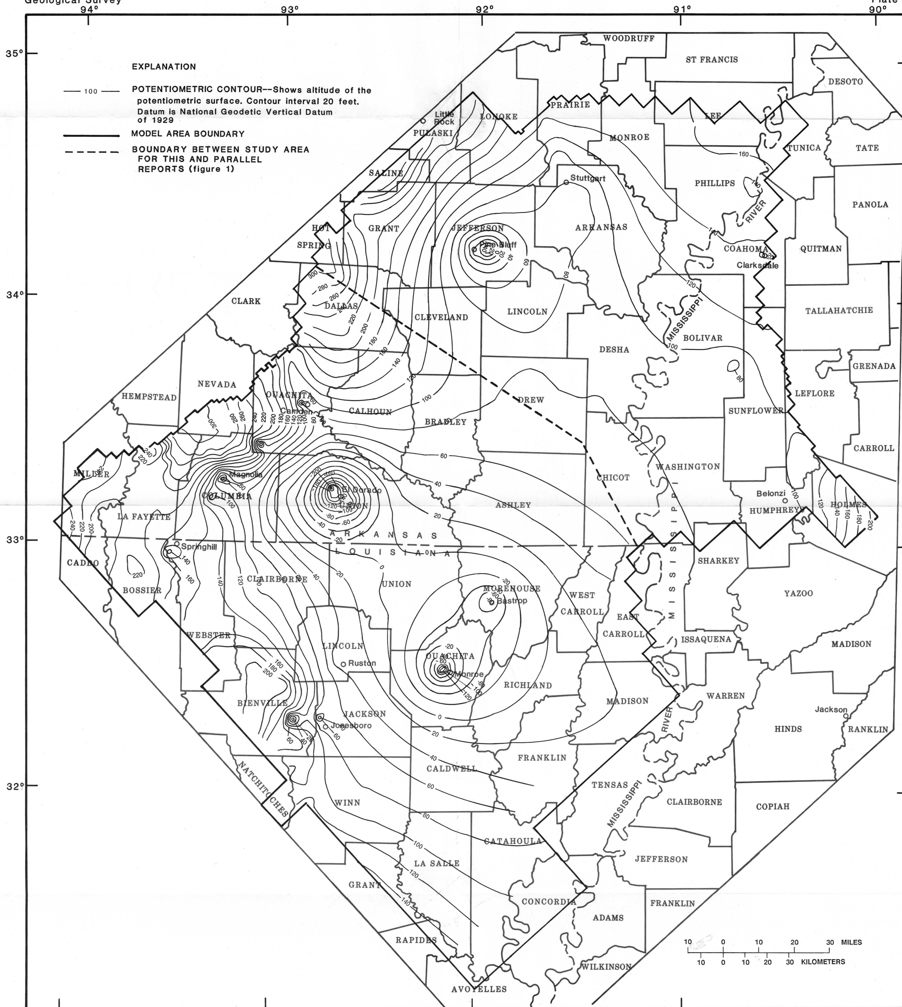
SIMULATED POTENTIOMETRIC SURFACE OF THE SPARTA AQUIFER, 1970
