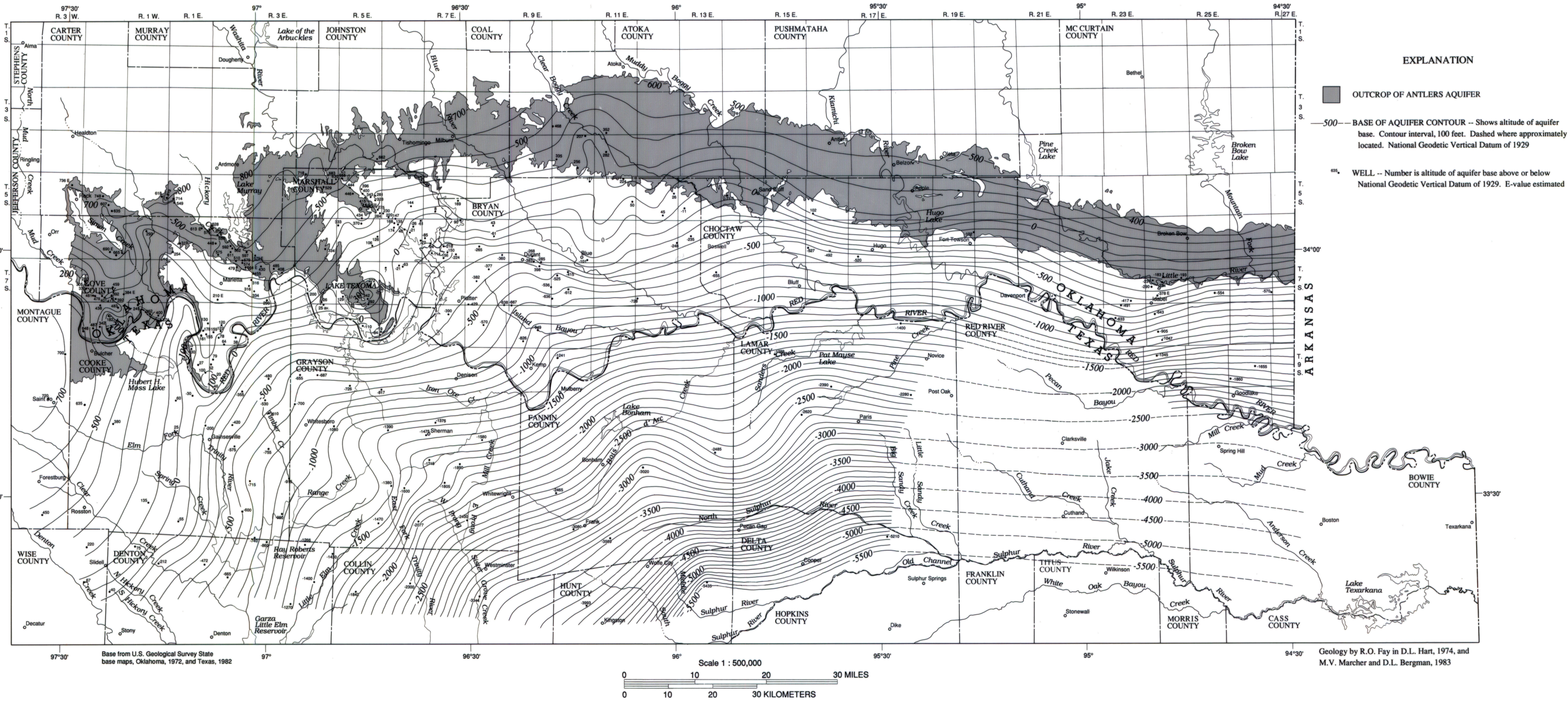
C. MAP SHOWING ALTITUDE OF THE BASE OF THE ANTLERS AQUIFER
