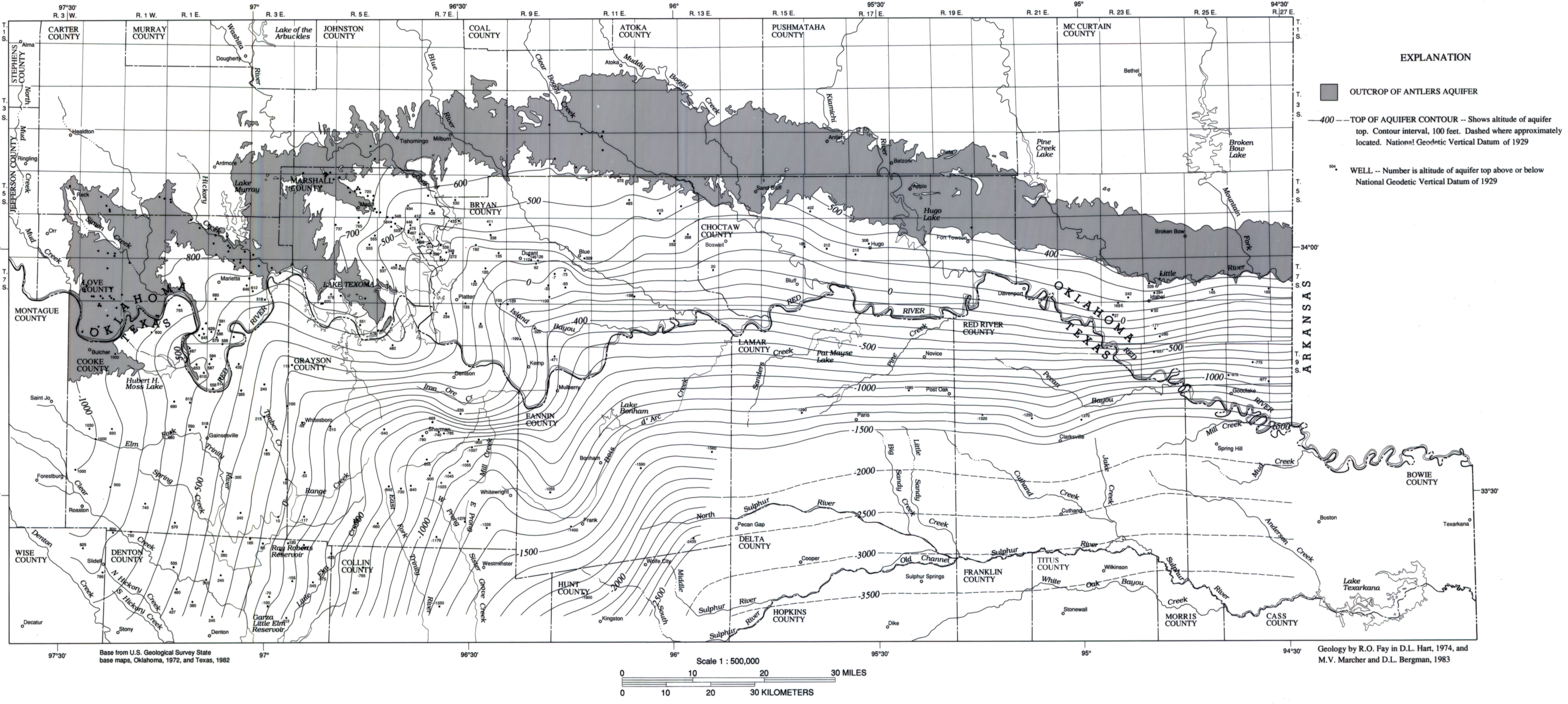
B. MAP SHOWING ALTITUDE OF THE TOP OF THE ANTLERS AQUIFER
