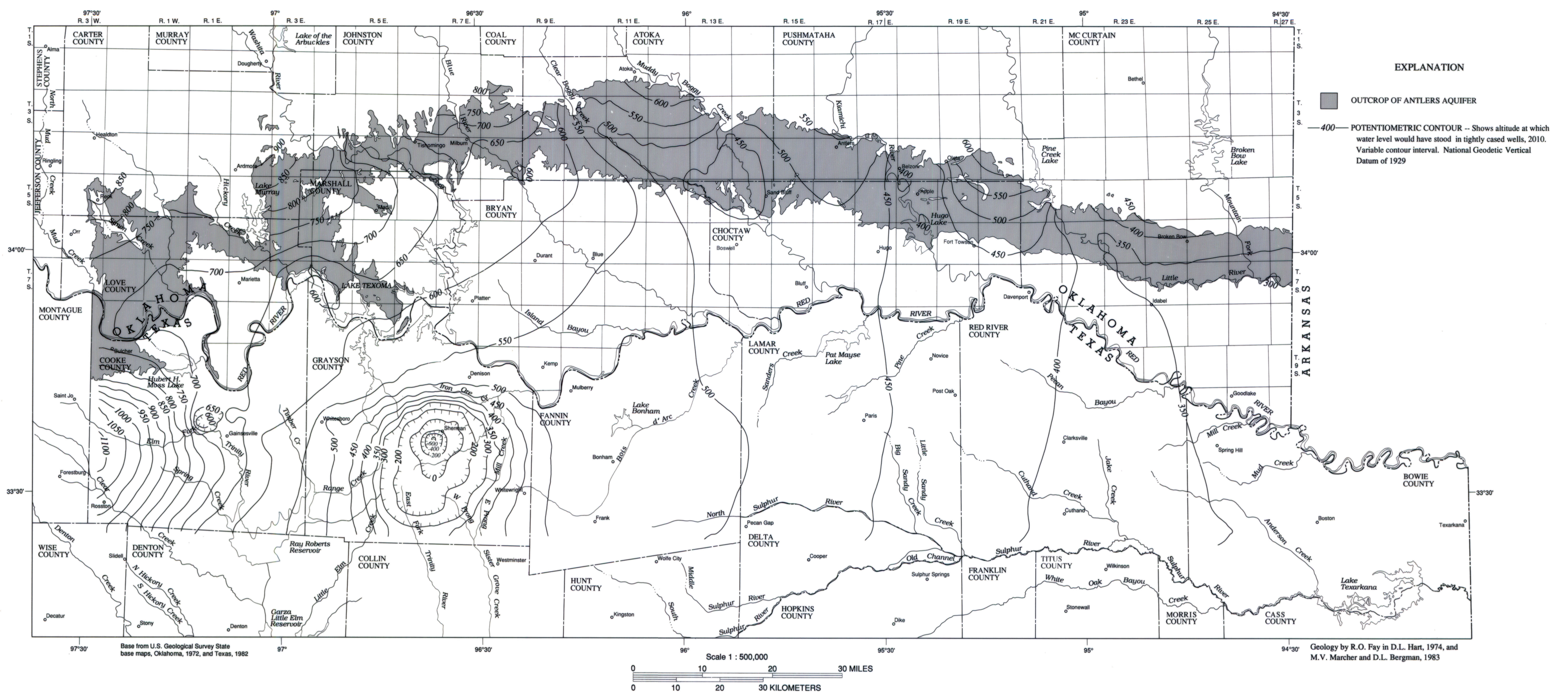
A. MAP SHOWING POTENTIOMETRIC SURFACE IN THE ANTLERS AQUIFER, 2010
