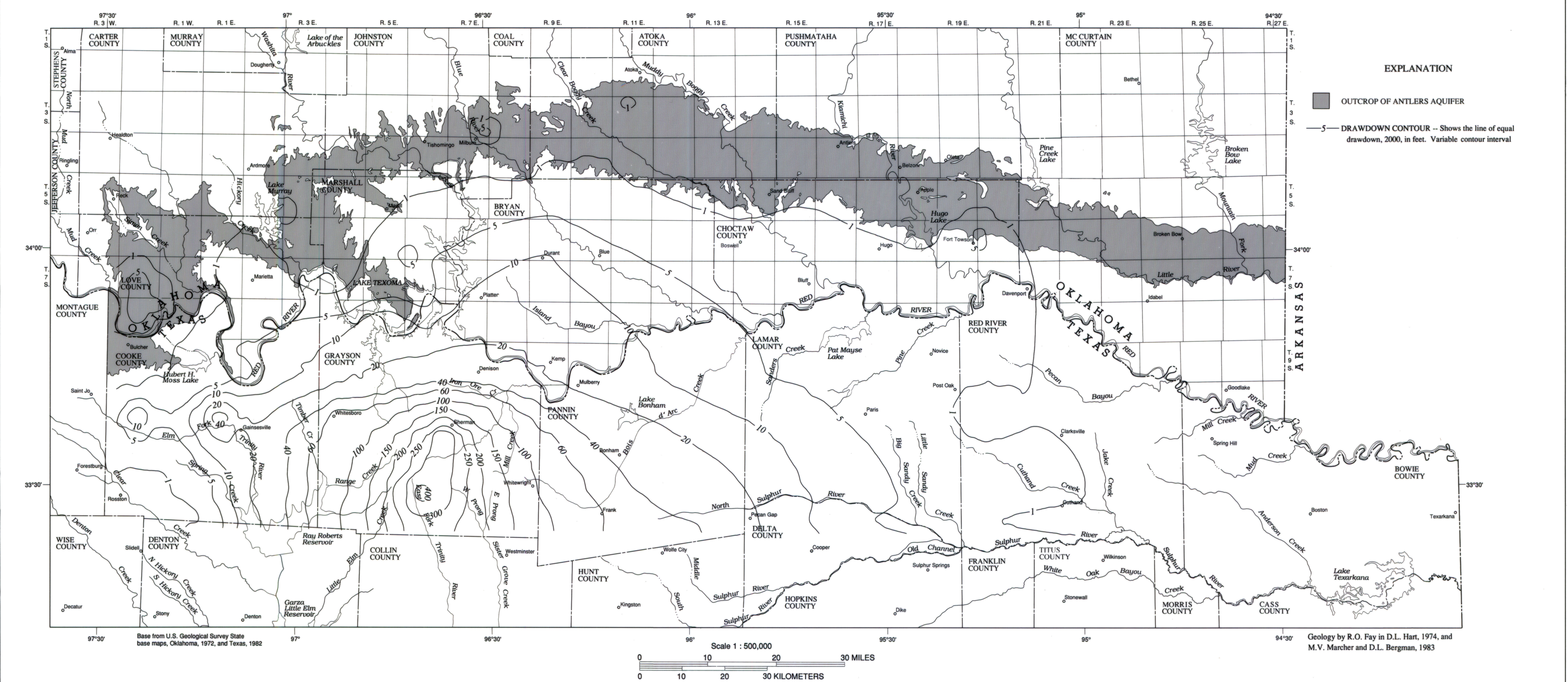
C. MAP SHOWING DRAWDOWN IN THE ANTLEERS AQUIFER, 2000
