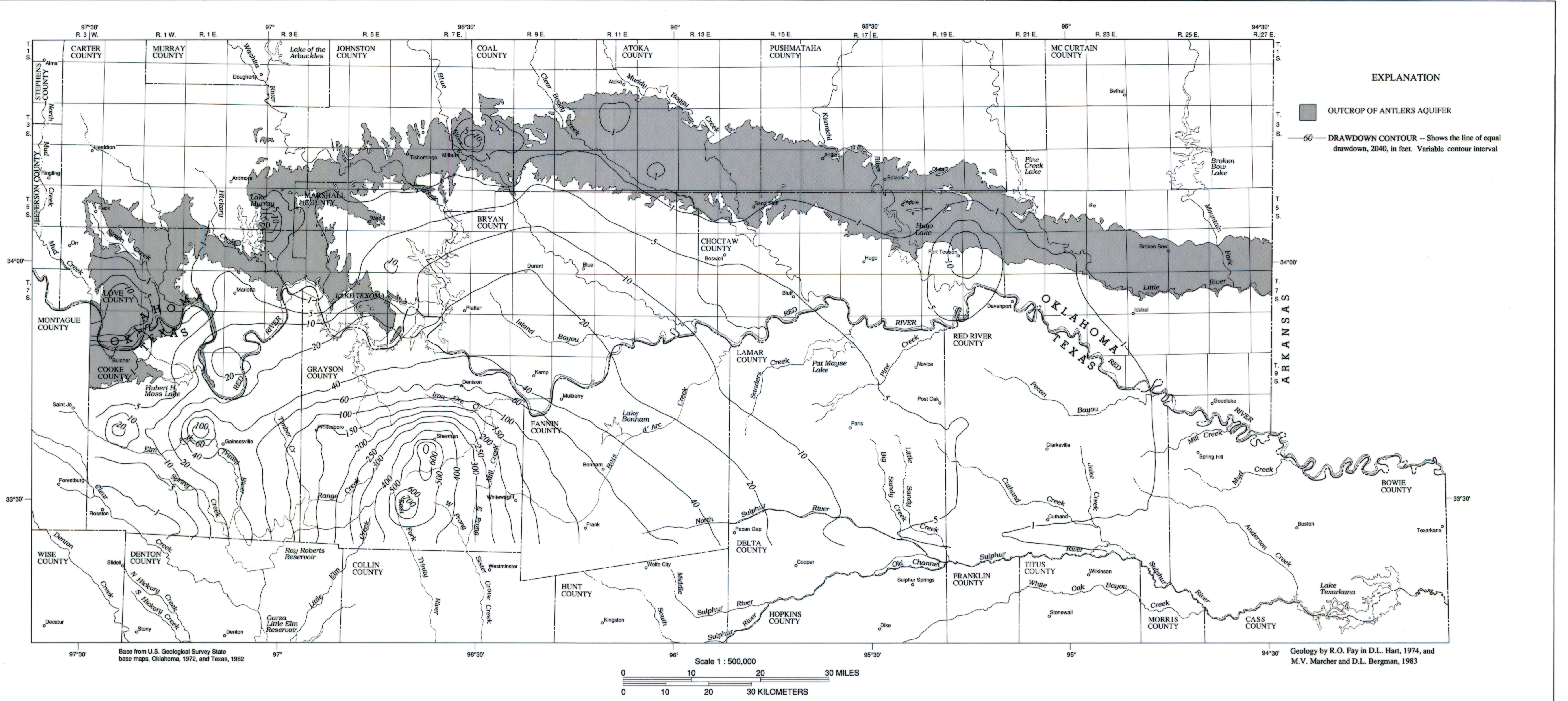
A. MAP SHOWING DRAWDOWN IN THE ANTLERS AQUIFER, 2040
