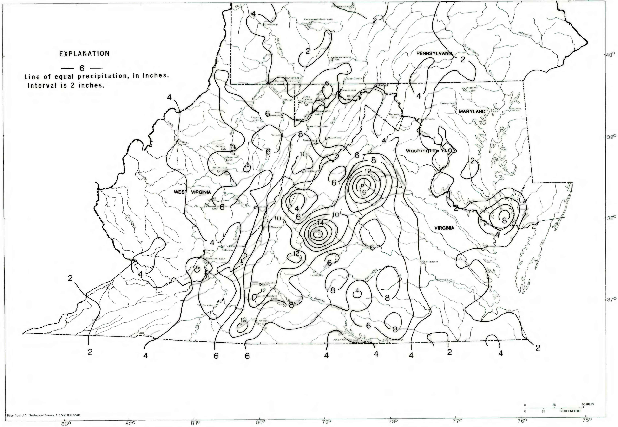
Figure 5.-- Total storm rainfall, October 31 - November 6, 1985.
