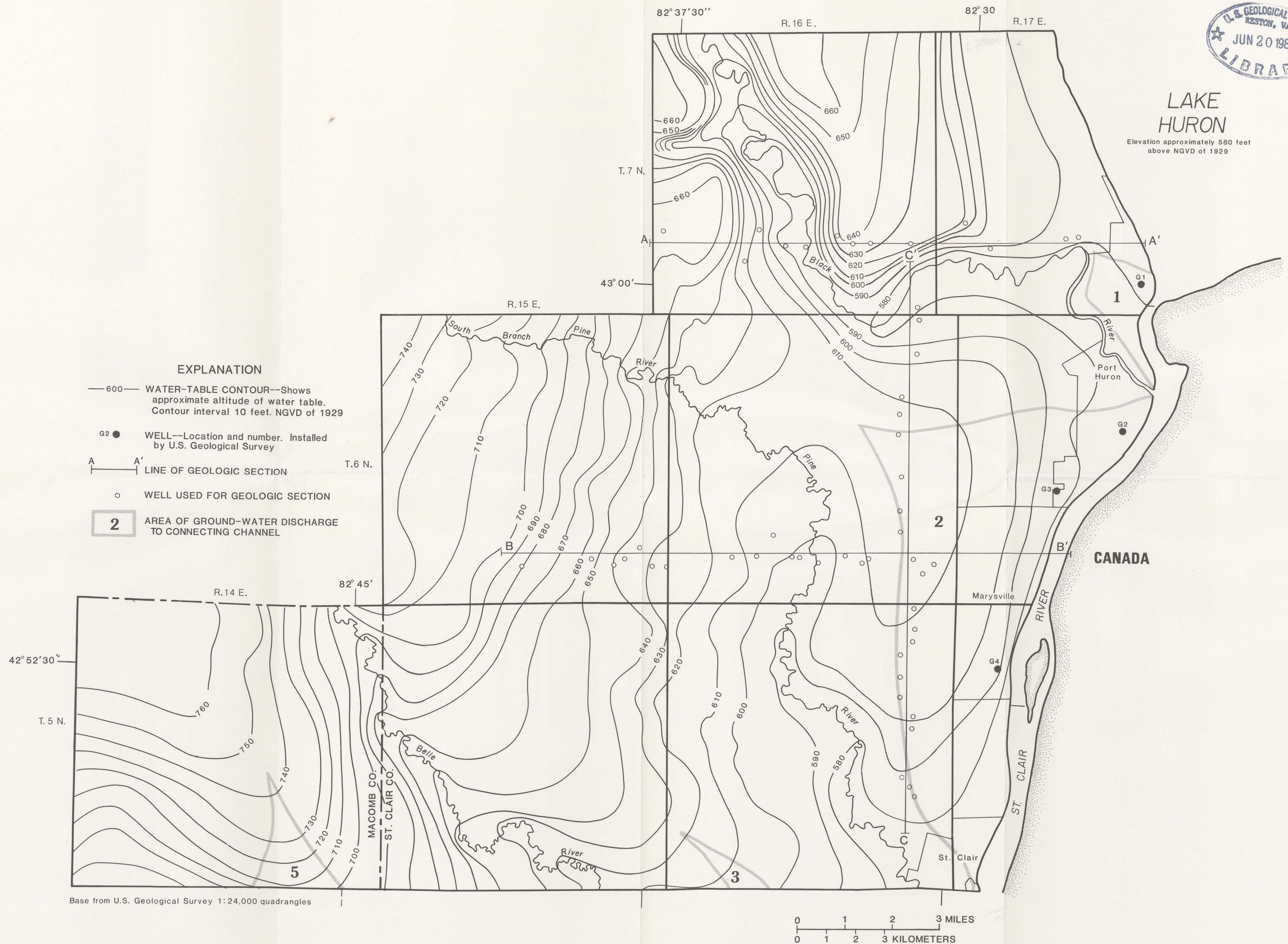
Water-table configuration, areas of ground-water discharge, and location of geologic sections in central St. Clair and northern Macomb Counties .
